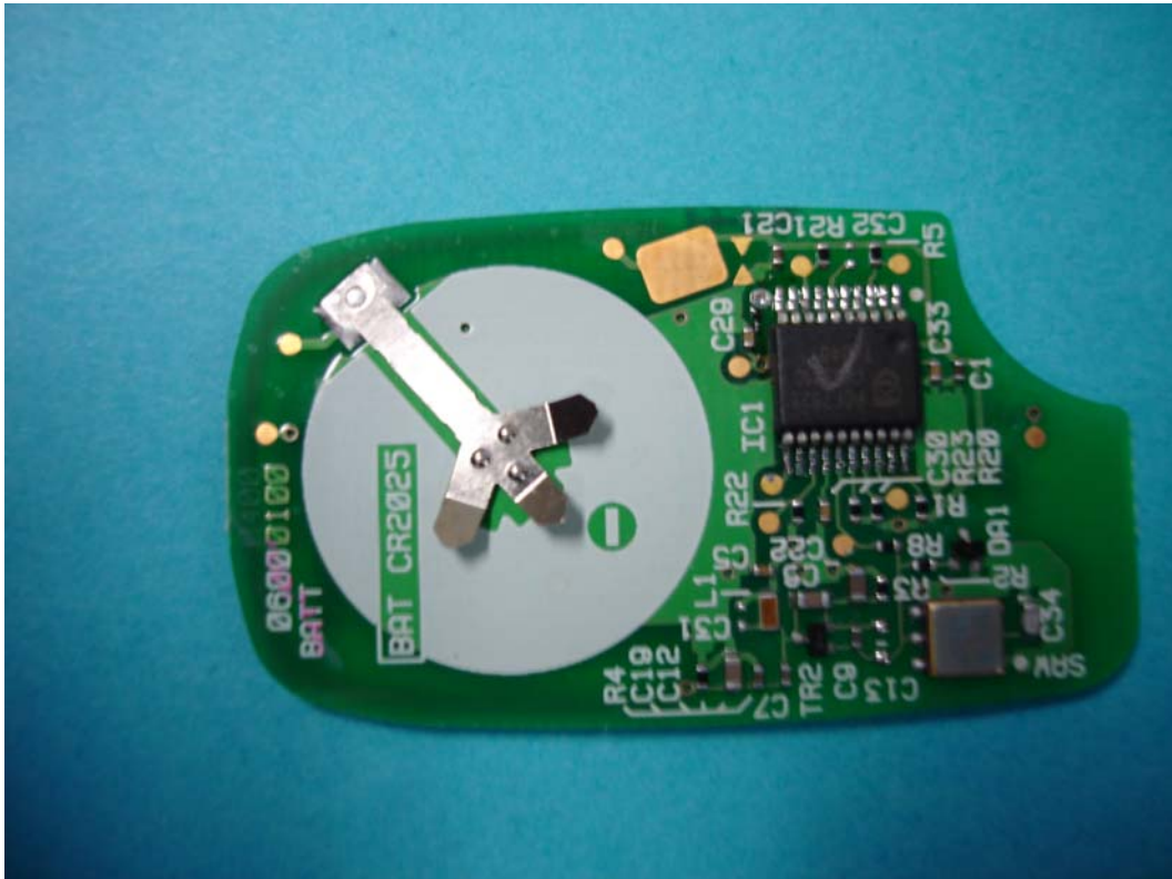
Circuit board <Front>
