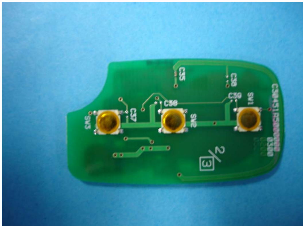
Circuit board <Rear >
