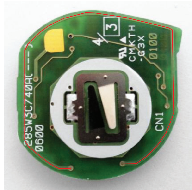
— ANTENNA PATTERN
