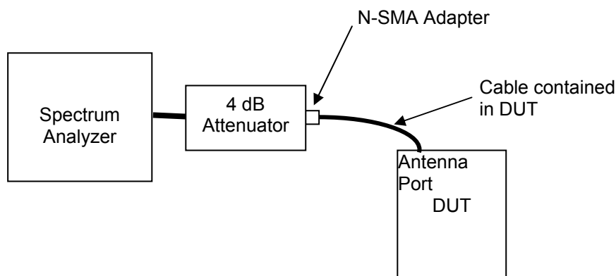
Figure I.6-1 - Setup Drawing
