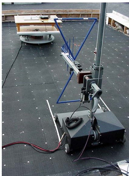
Photograph F.7-4 - Mobile - 3 m Bilog Setup
