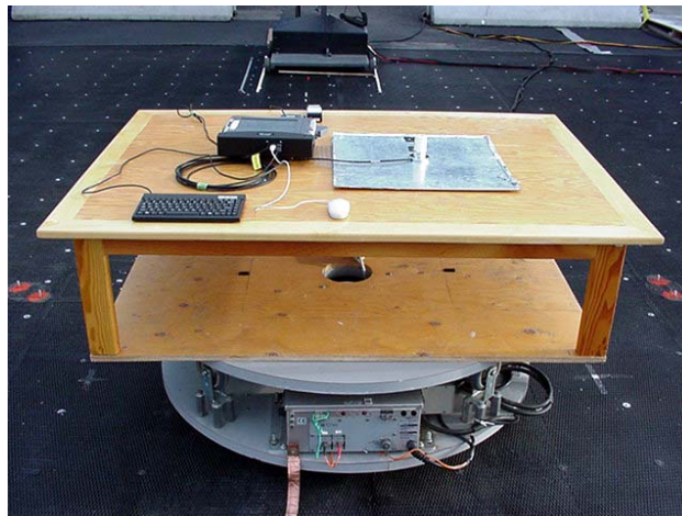
Photograph F.7-2 - Mobile DUT Configuration
