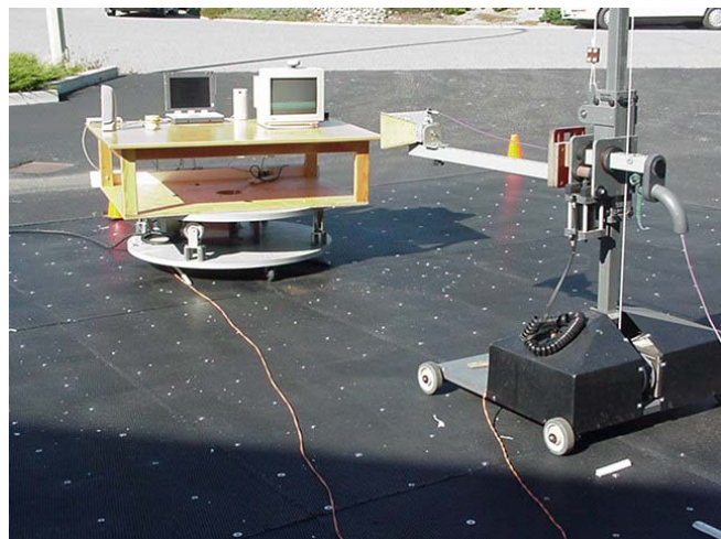
Photograph C-3– 3115 Horn Antenna
