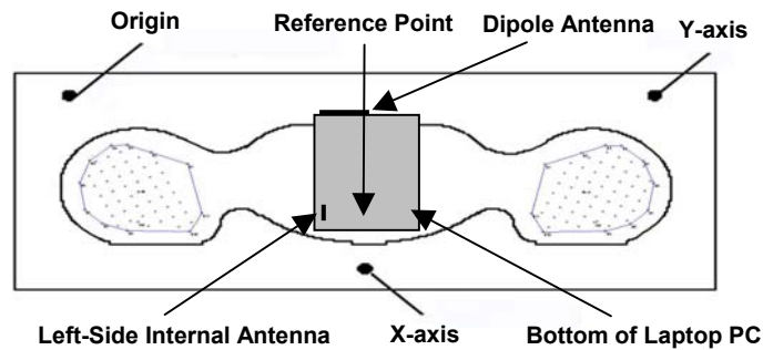
Figure 4. Phantom Reference Point & DUT Positioning Bottom Left Side of Laptop PC (LCD Display Closed)- Left-Side Internal Antenna
