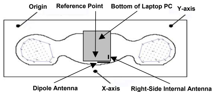
Figure 5. Phantom Reference Point & DUT Positioning Bottom Right Side of Laptop PC (LCD Display Closed)- Right-Side Internal Antenna
