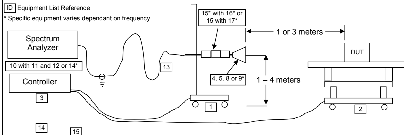
Figure C.6-1 - Setup Drawing
