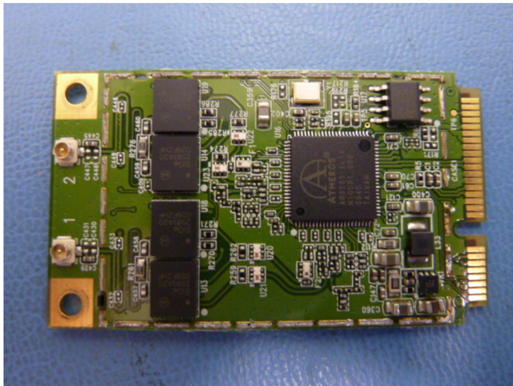
Figure 2: Top View (without shielding)
