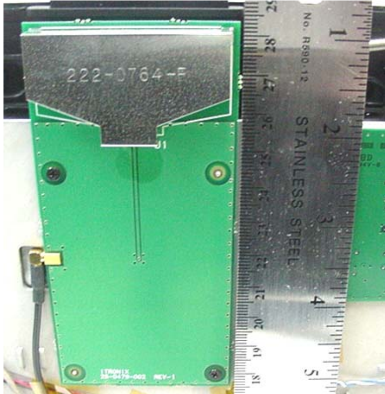
Distance from Laptop PC Base to Antenna (LCD Display Lid Open)
