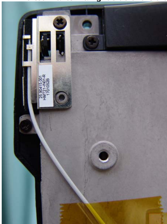
WLAN Inverted F antenna right side of the display
