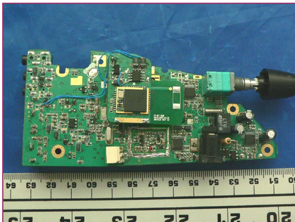
EUT – Main and Sub-PCBA Component Board View-3
