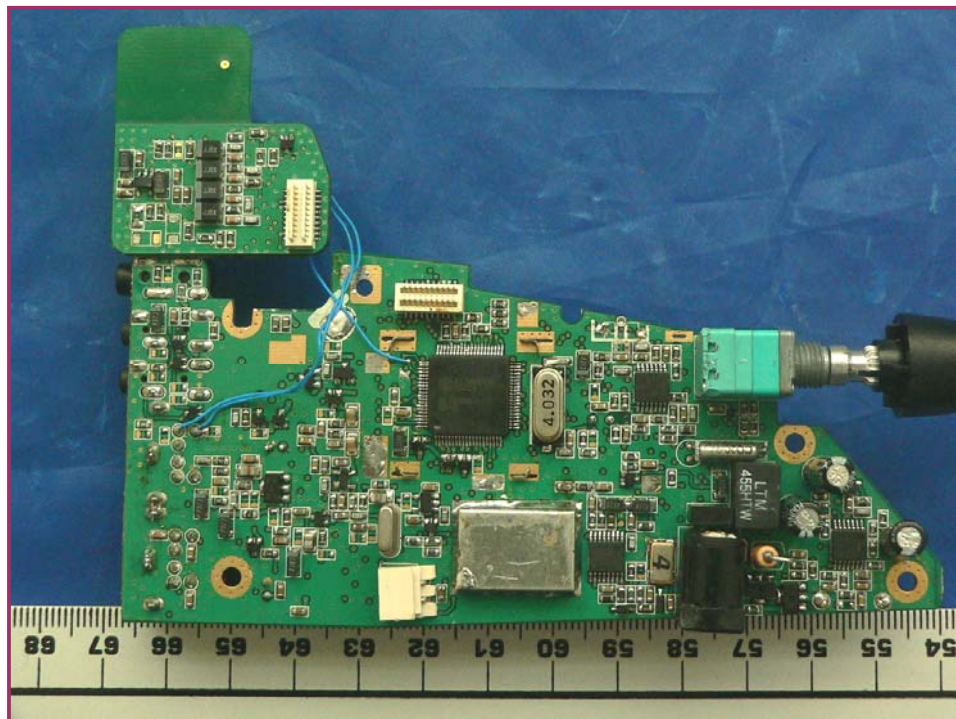
EUT – Main and Sub-PCBA Component Board View-2
