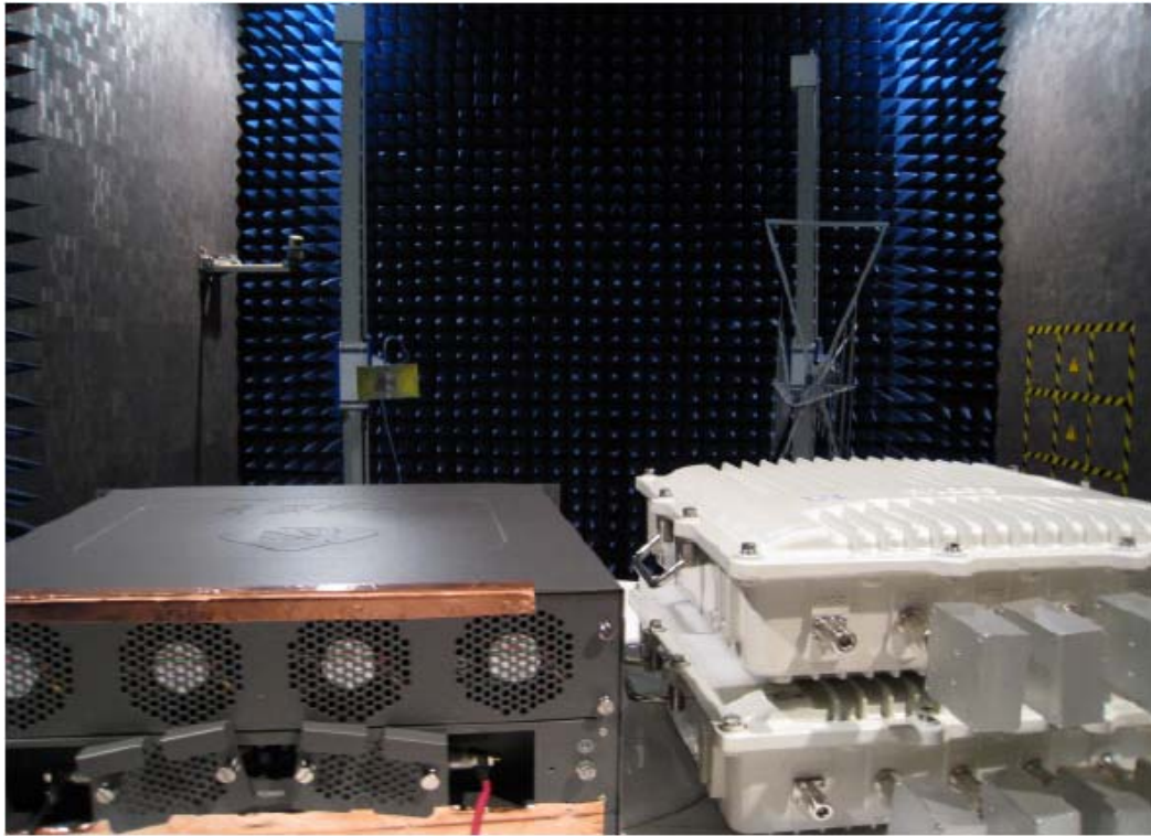
Radiated Spurious Emissions Test setup
