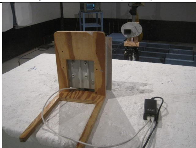
Radiated Spurious Emissions 18-40GHz (20dBi Ant) – Rear View
