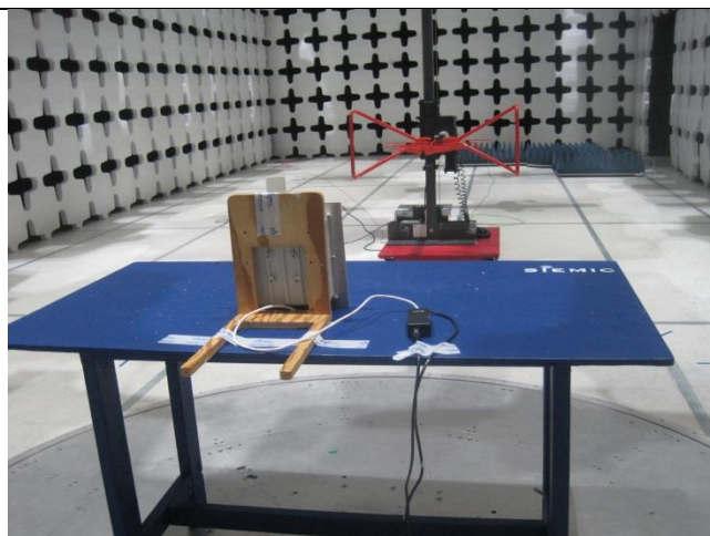
Radiated Spurious Emissions <1GHz (20dBi Ant) – Rear View
