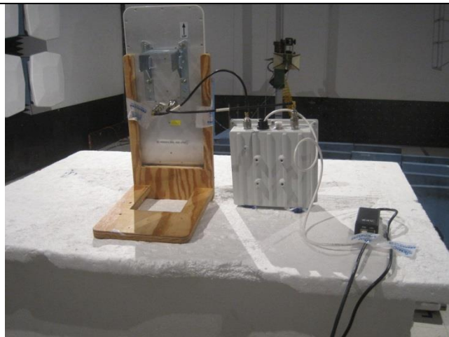
Radiated Spurious Emissions 1-18GHz (16dBi Ant) – Rear View
