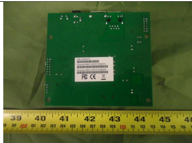
EUT – Main PCBA Bottom View
