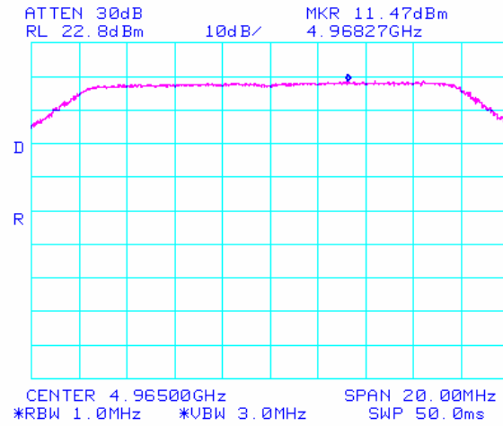
Plot 6: Peak Power Spectral Density 20MHz Bandwidth
