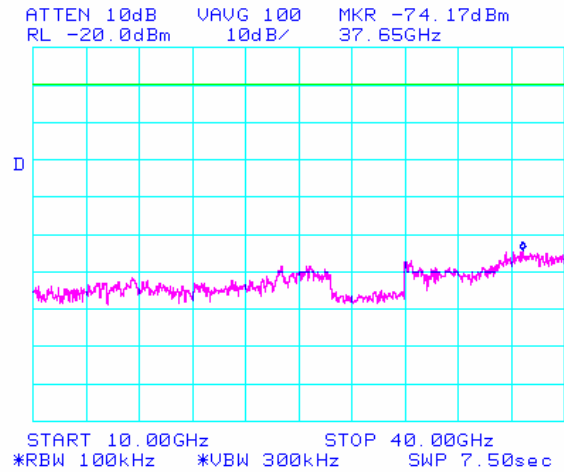
Plot 12: Conducted Spurious 5MHz BW 3 of 3
