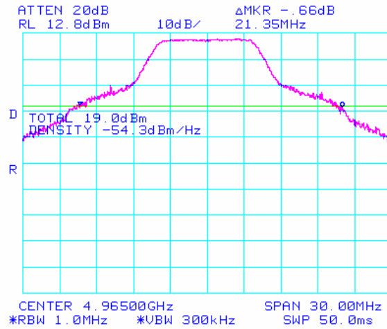
Plot 2: Peak Power 10MHz Bandwidth
