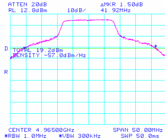
Plot 3: Peak Power 20MHz Bandwidth
