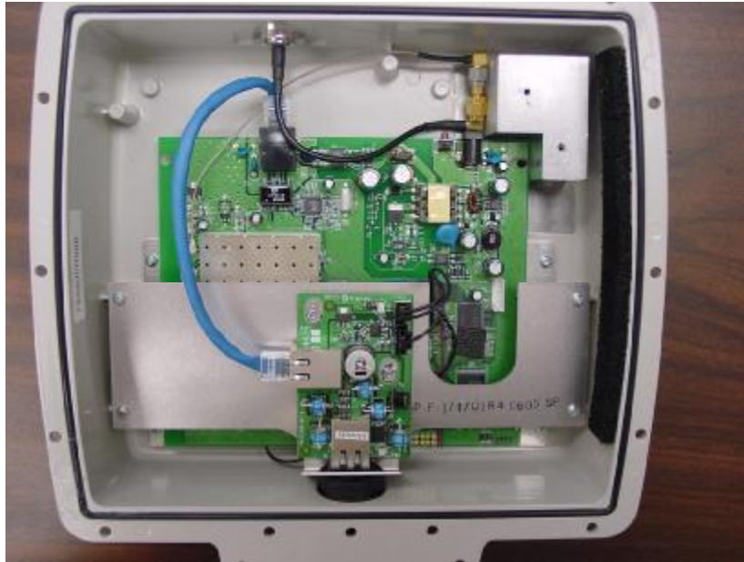
Photo 1: Assembly
