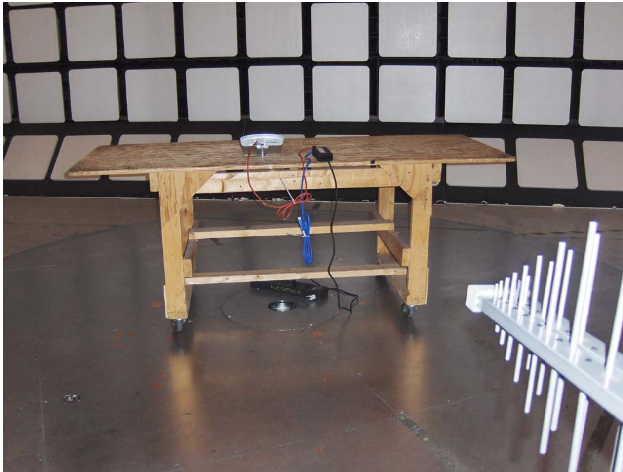
Plot #3: Test setup for Radiated Emissions in Semi-Anechoic Chamber
