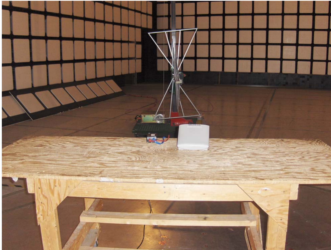
Plot #4: Test setup for Radiated Emissions in Semi-Anechoic Chamber
