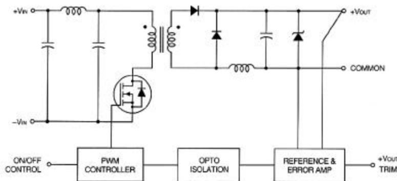
Figure 1. Simplified Schematic
