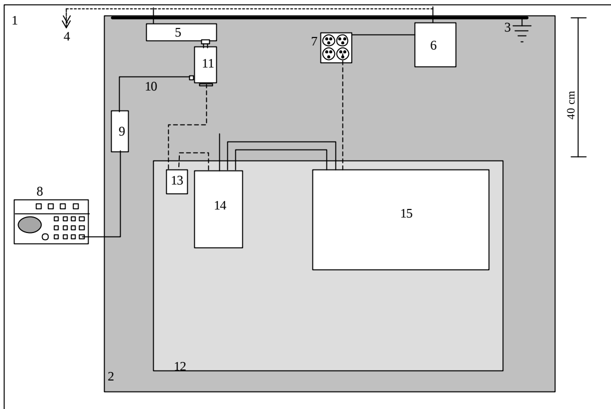
Figure 5. Conducted Emissions Test Setup Diagram
