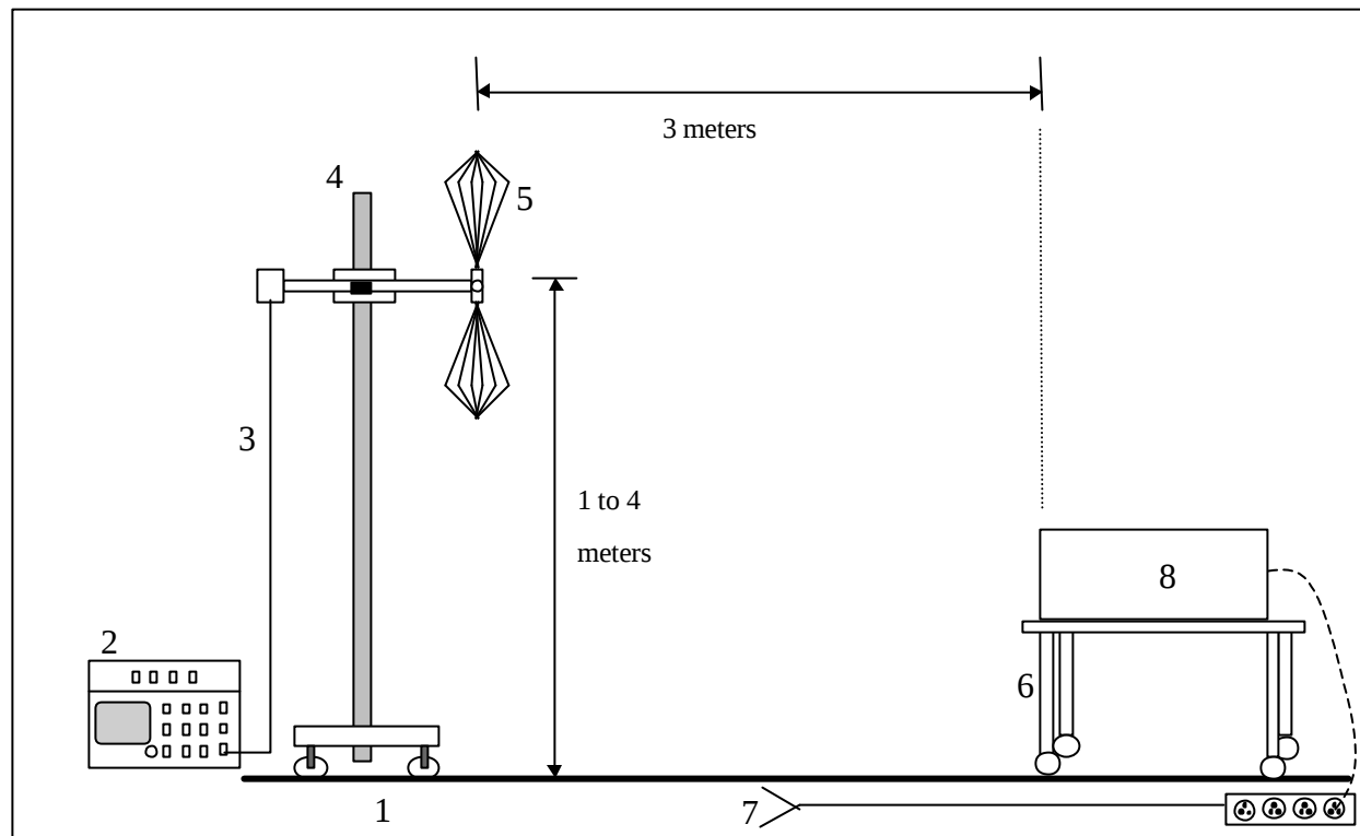
Figure 7. Radiated Emissions (OATS) Test Setup Diagram
