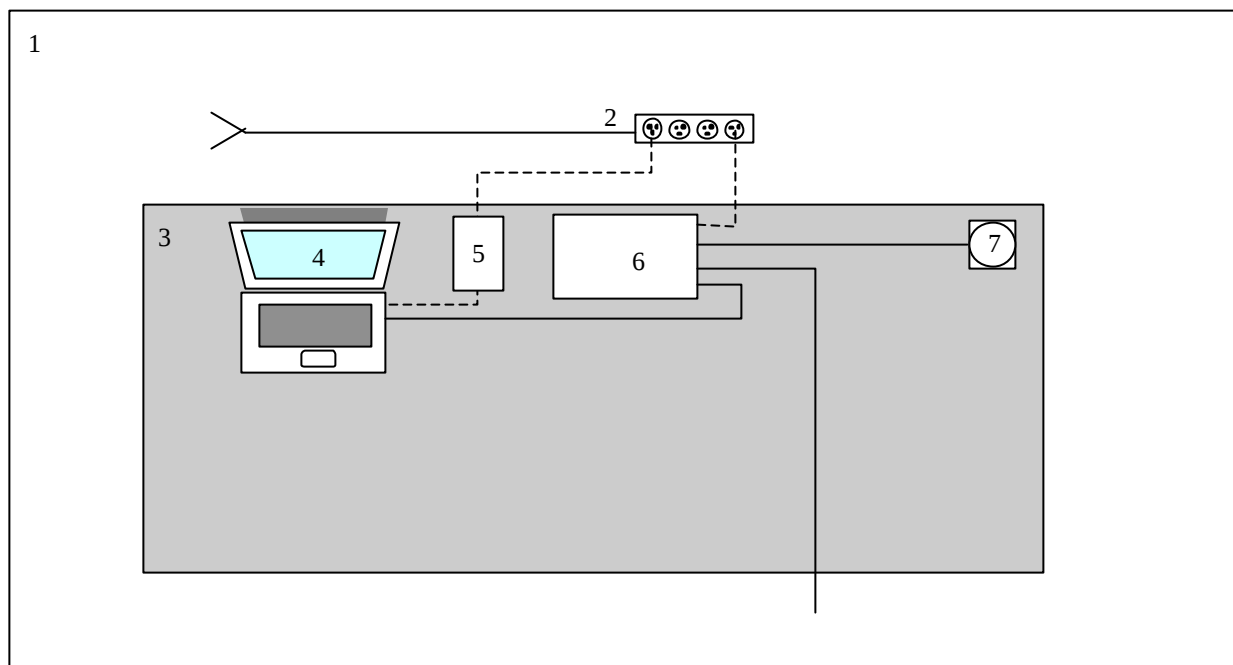
Figure 4. General EUT Test Setup Diagram
