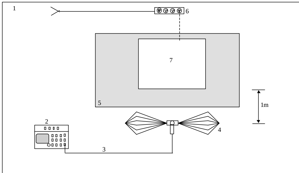
Figure 6. Radiated Emissions Frequency ID Test Setup Diagram
