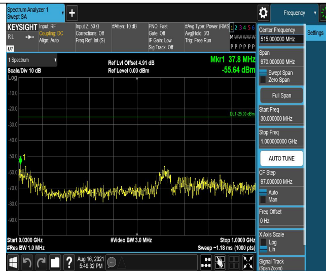
Band7-10MHz-16QAM-21400-50RB#0-Range1:30~1000MHz
