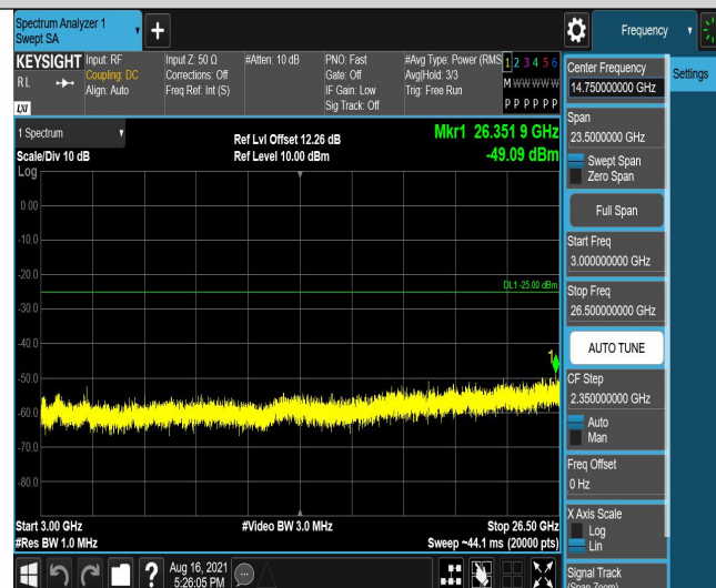
Band7-5MHz-16QAM-21100-25RB#0-Range3:3000~26500MHz
