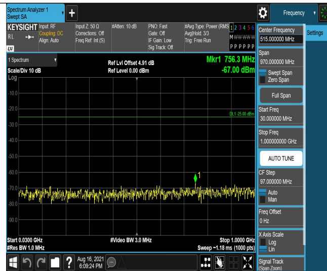
Band7-15MHz-QPSK-20825-75RB#0-Range1:30~1000MHz
