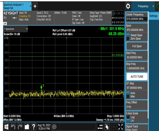
Band7-5MHz-16QAM-21100-25RB#0-Range1:30~1000MHz
