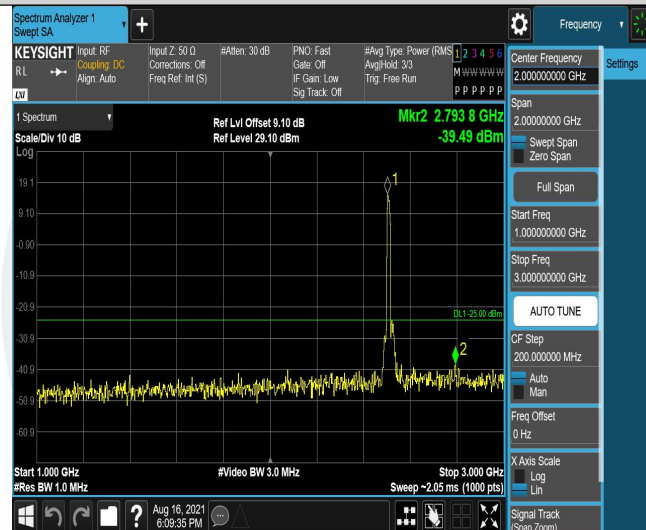
Band7-15MHz-QPSK-20825-75RB#0-Range2:1000~3000MHz
