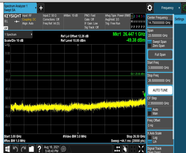
Band7-10MHz-16QAM-21100-50RB#0-Range3:3000~26500MHz
