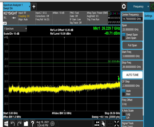
Band7-5MHz-16QAM-20775-25RB#0-Range3:3000~26500MHz
