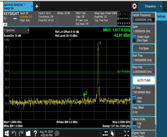
Band4-5MHz-16QAM-20175-25RB#0-Range2:1000~2000MHz
