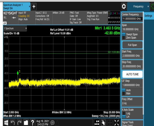
Band4-3MHz-16QAM-20175-6RB#0-Range3:2000~20000MHz
