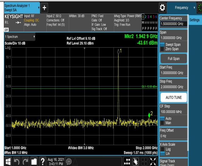
Band4-3MHz-16QAM-20175-6RB#0-Range2:1000~2000MHz
