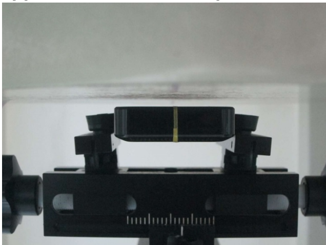
Front of the DUT with Phantom 0.5 cm Gap
