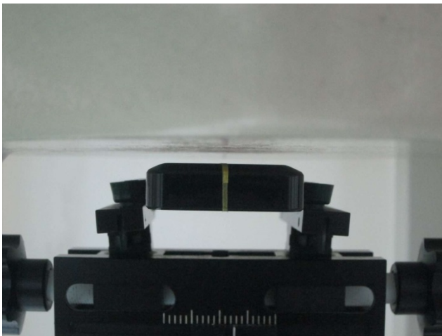
Back of the DUT with Phantom 0.5 cm Gap
