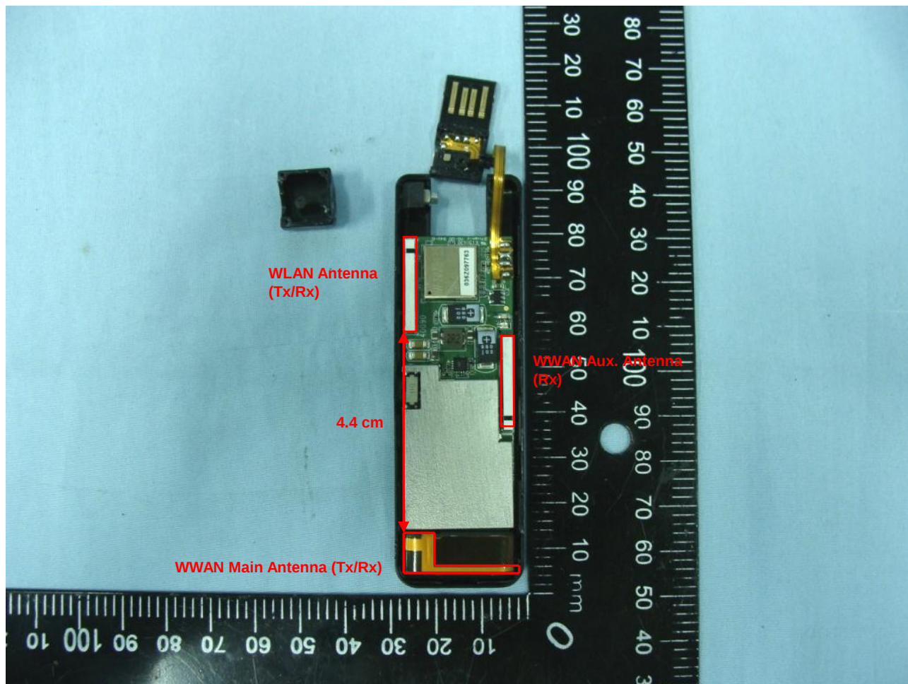
Antenna Location
