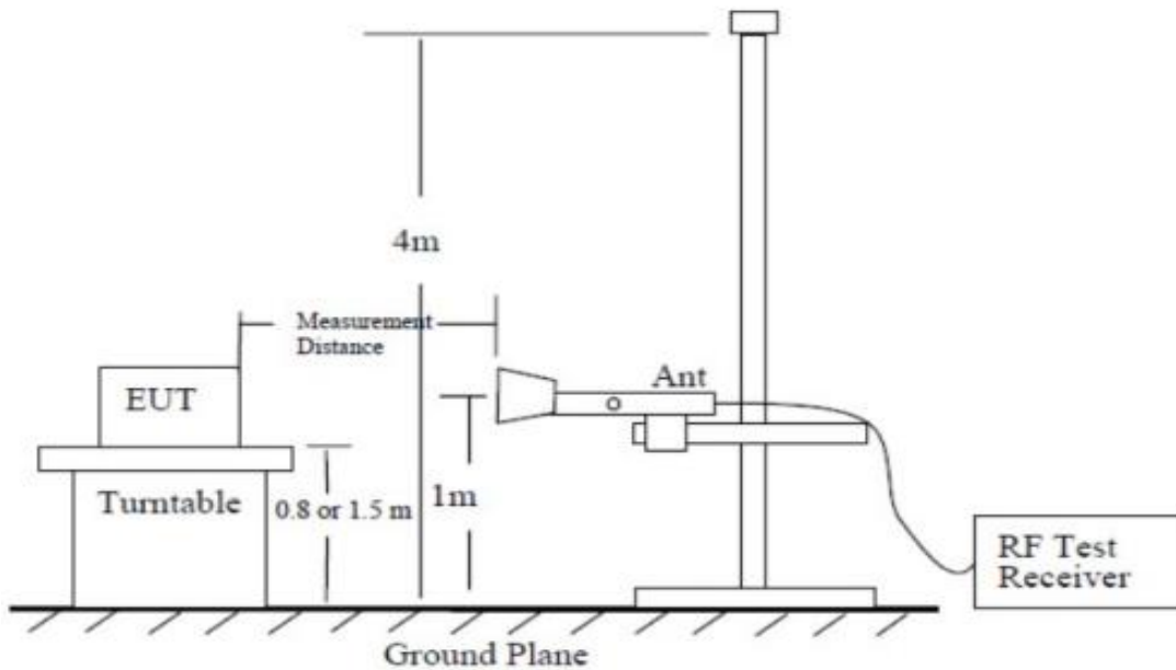
Test site-up for radiated ERP and/or EIRP measurements
