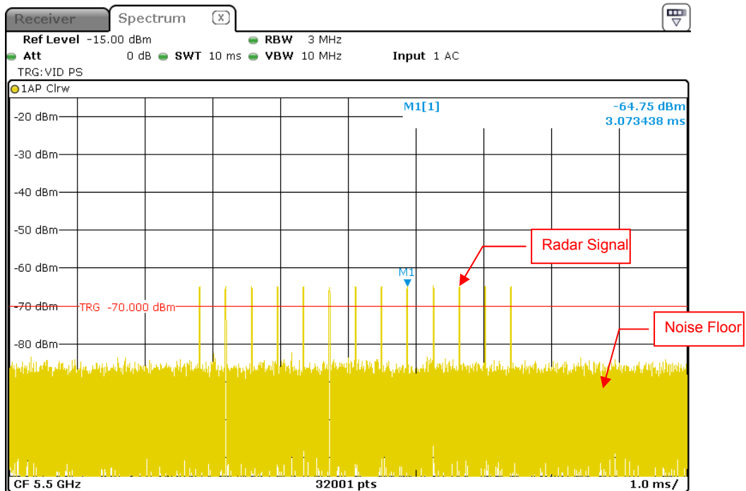
Radar Signal 4
