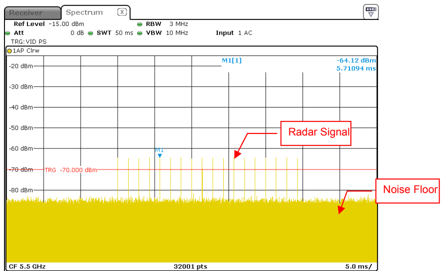
Radar Signal 0
