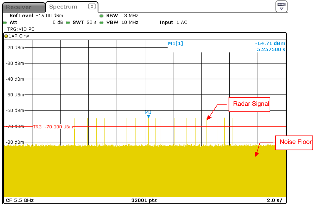
Radar Signal 5
