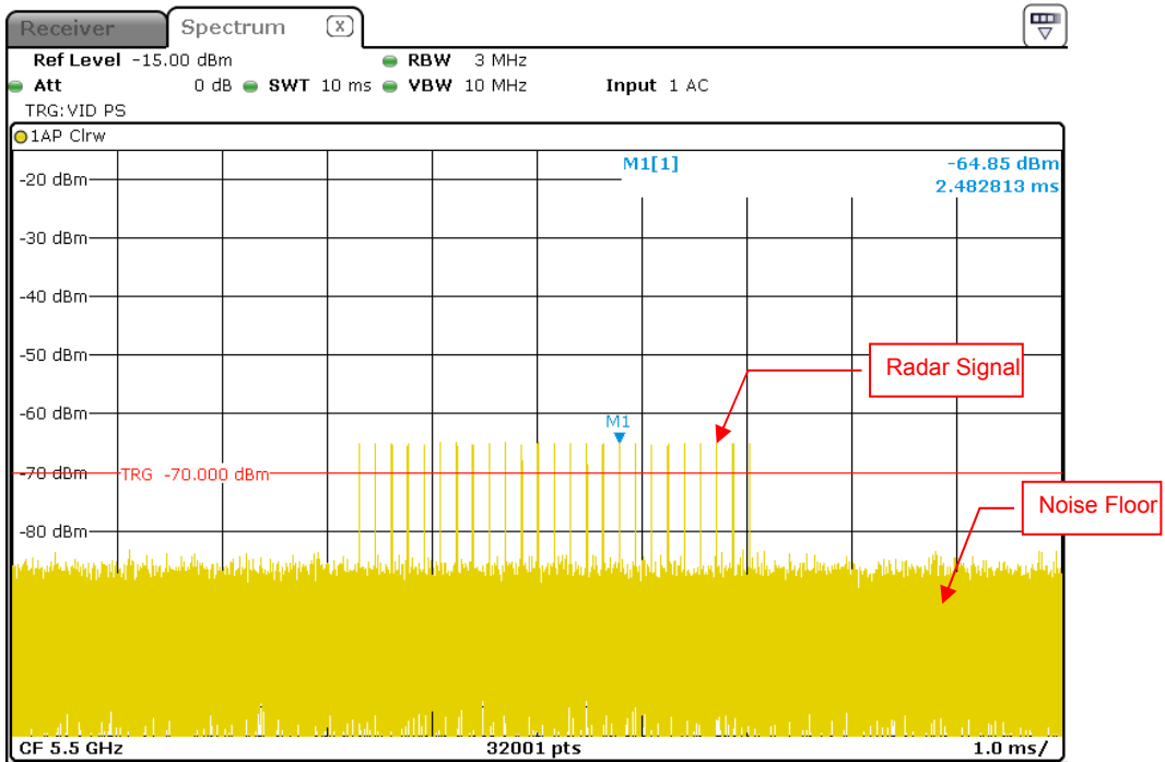
Radar Signal 2
