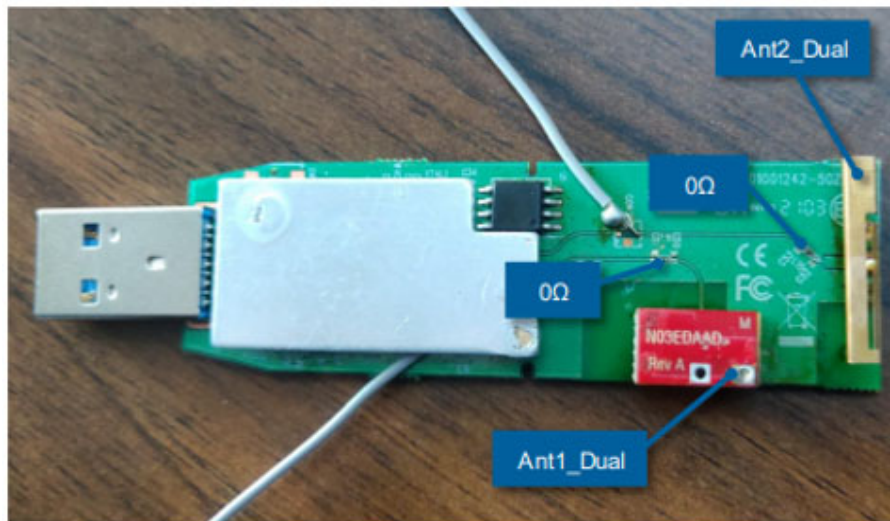
<Rear Face View>
