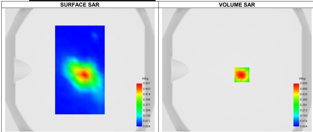
Maximum location: X=8.00, Y=-8.00 ; SAR Peak: 0.97 W/kg
