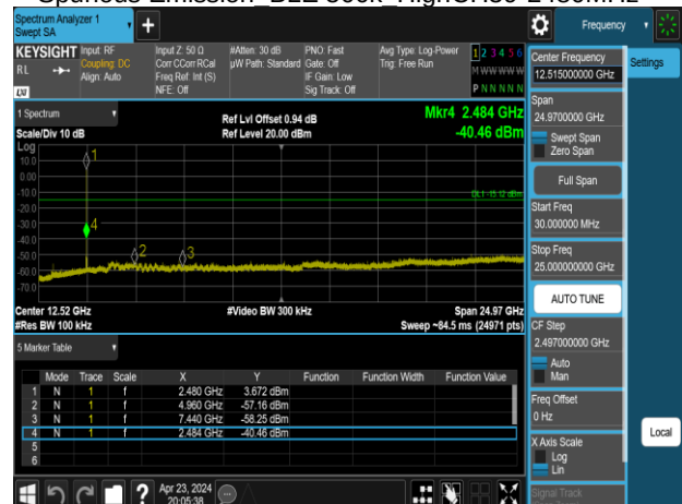
Spurious Emission BLE 500k HighCH39-2480MHz
