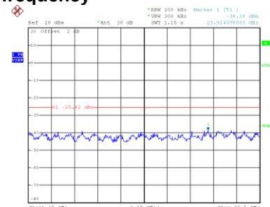
CH06 – 10th Harmonic of the fundamental frequency
