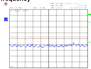
CH09 – 10th Harmonic of the fundamental frequency
