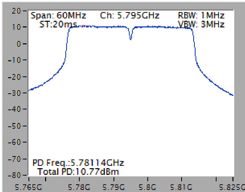
Power Density Plot on Configuration IEEE 802.11ac MCS0/Nss1 VHT40 / Ant. 2 + Ant. 3 + Ant. 4 / 5795 MHz
