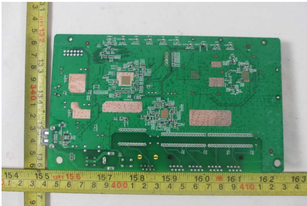
Main board
