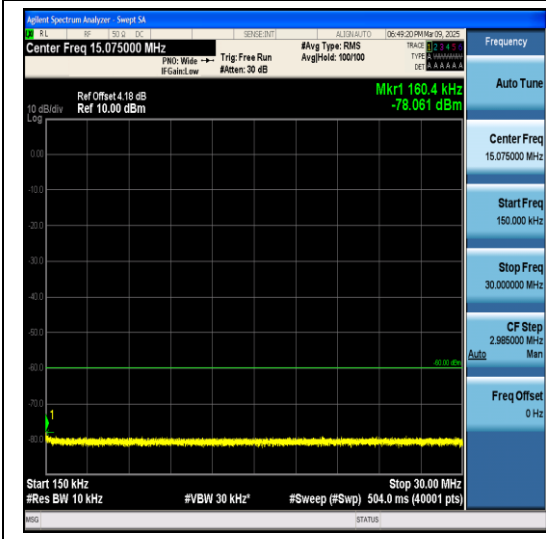
Band40(2345-2360)-10MHz-QPSK-39200-1RB#0-0.15~30-PASS
