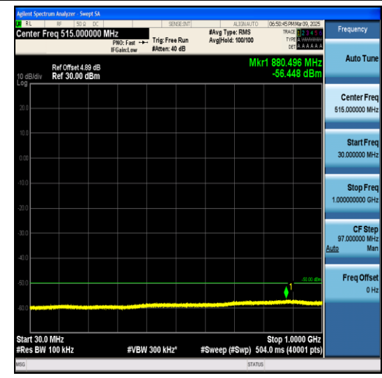
Band40(2345-2360)-10MHz-QPSK-39200-1RB#0-30~1000-PASS
