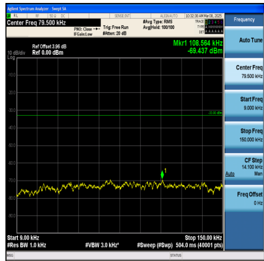
Band5-5MHz-QPSK-20525-1RB#0-0.009~0.15-P ASS
