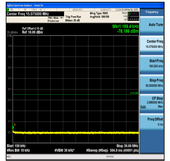
Band7-5MHz-QPSK-21100-1RB#0-0.15~30-PASS
