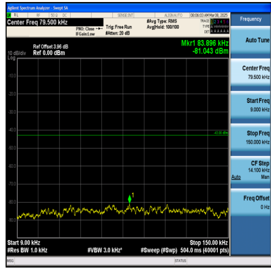
Band4-5MHz-QPSK-20175-1RB#0-0.009~0.15-P ASS
