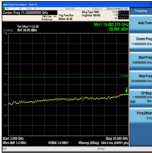
Band4-5MHz-QPSK-19975-1RB#0-3000~20000-P ASS
