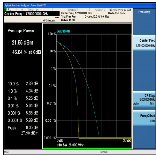
Band66-10MHz-QPSK-132622-50RB#0-PASS
