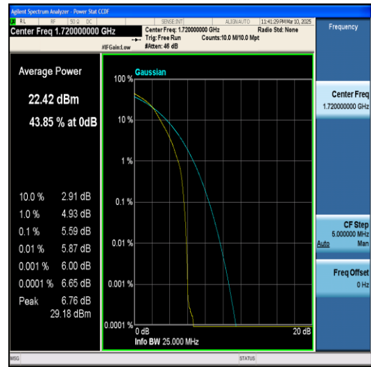
Band66-20MHz-QPSK-132072-100RB#0-PASS
