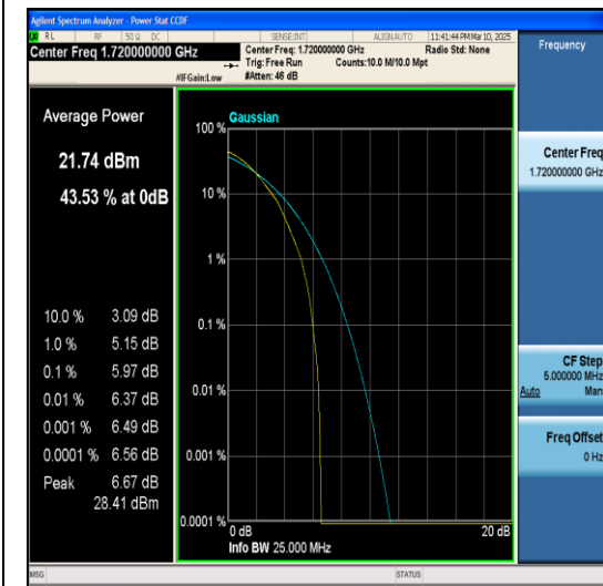
Band66-20MHz-64QAM-132072-1RB#0-PASS
