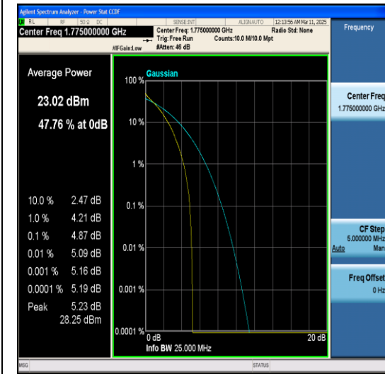
Band66-10MHz-64QAM-132622-1RB#0-PASS
