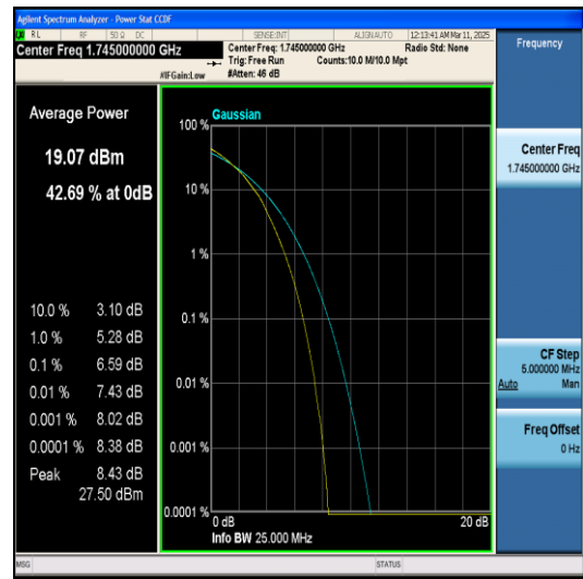
Band66-10MHz-16QAM-132622-1RB#0-PASS
