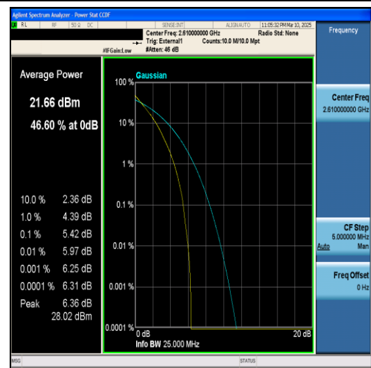
Band38-20MHz-QPSK-38150-100RB#0-PASS
