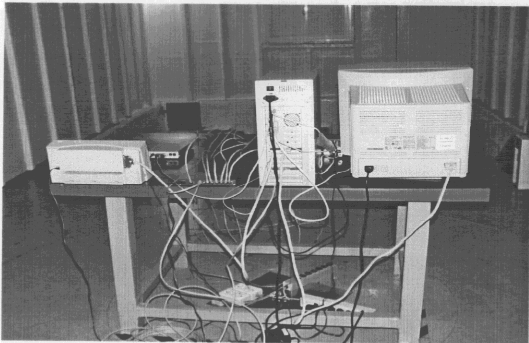
Mode2:Back View of Radiated Test (Maximum Testing Configuration)
