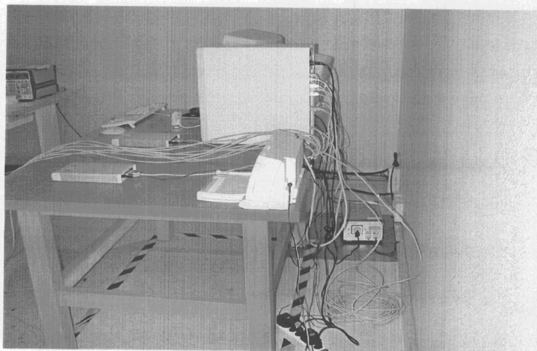
Model: Back View of Conducted Test ( Maximum Testing Configuration)
