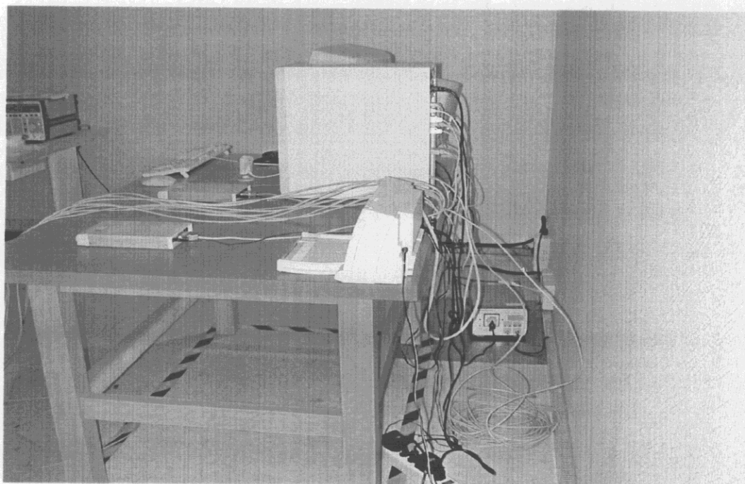
Mode2:Back View of Conducted Test ( Maximum Testing Configuration)
