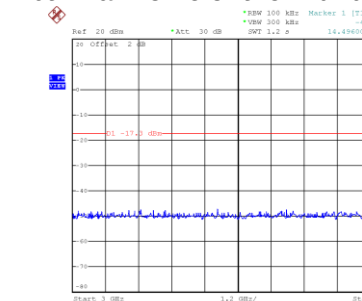
CH19 – 10th Harmonic of the fundamental frequency
