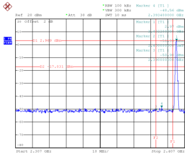
Bandedge CH00 (Lower)
