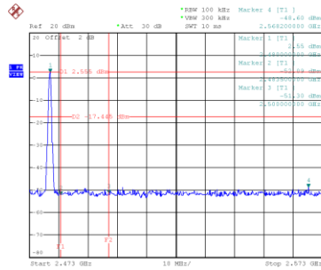
Bandedge CH39 (Upper)
