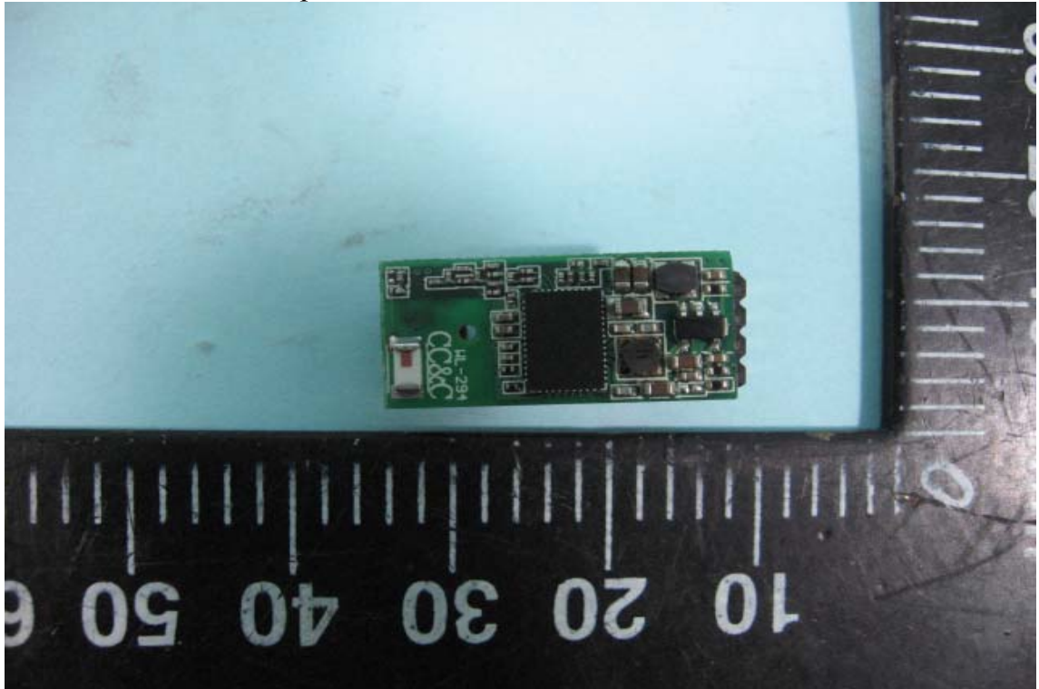
10. Wi-Fi Module Component View of PCB
