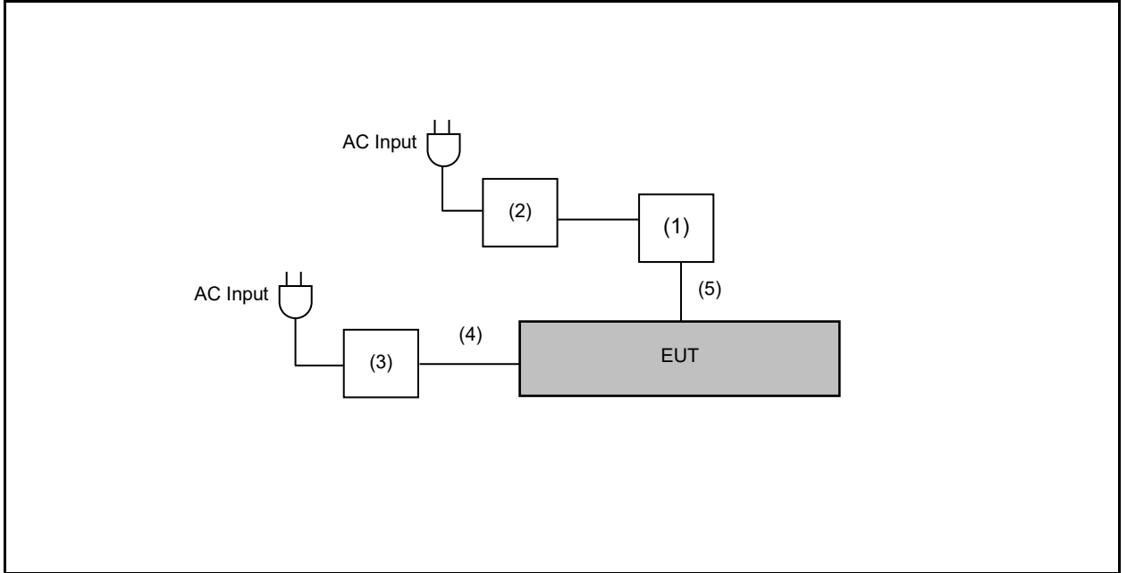
Conduction Emission
