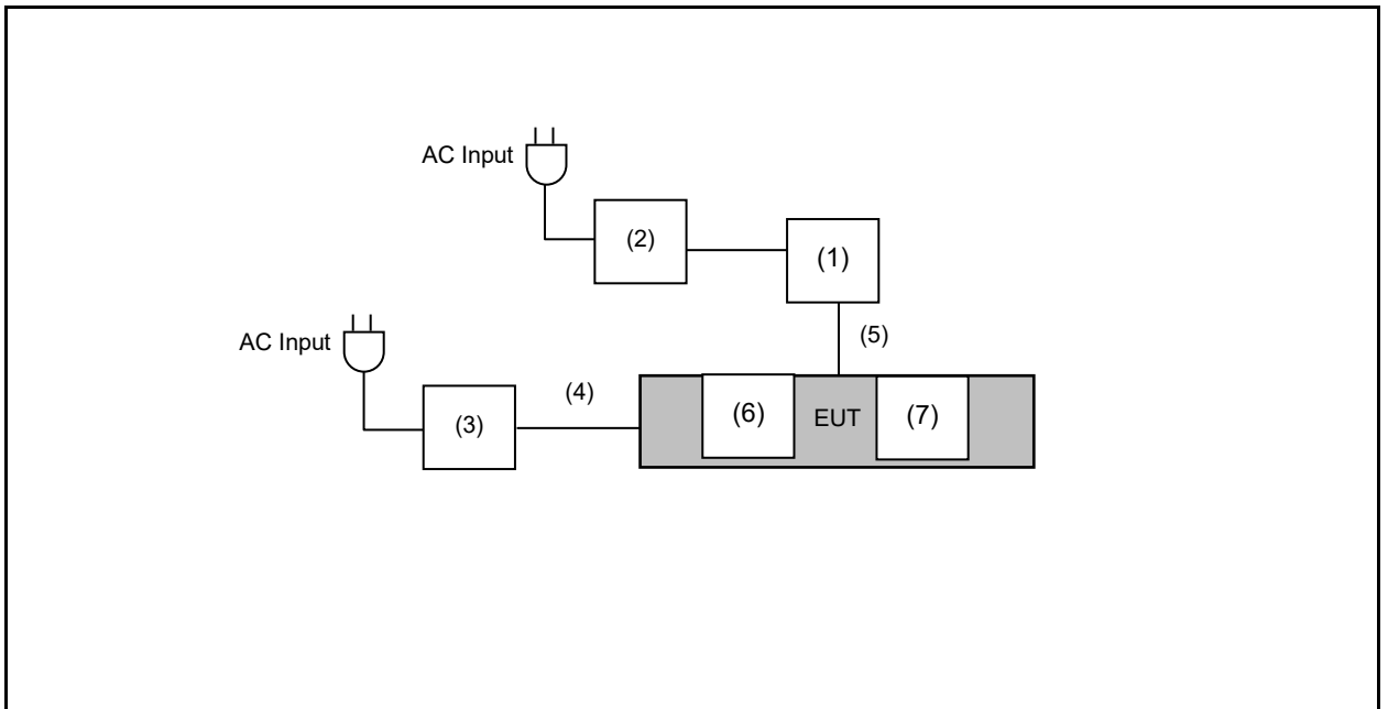
Conduction Emission
