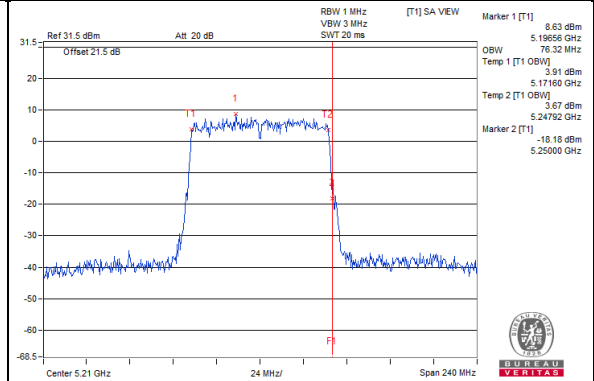
802.11ac(VHT80)_Chain0 / CH42
