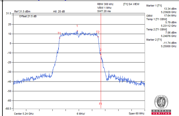
802.11ac(VHT20)_Chain0 / CH48
