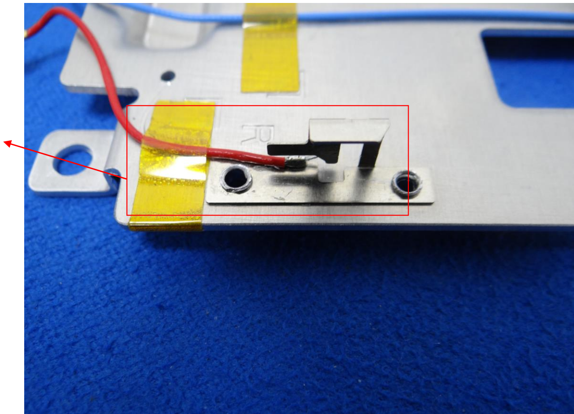
ANT 5 For Wifi 6E
