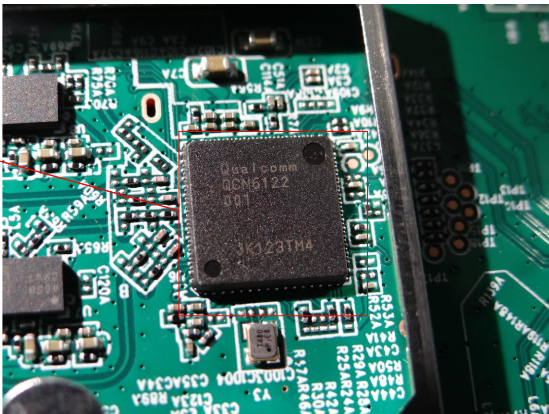
RF Chip For Wifi 6E
