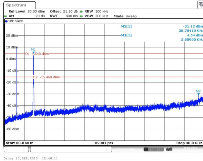
Conducted Emission Plots of Antenna port 1
