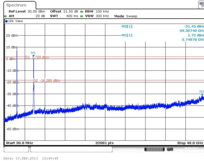
Conducted Emission Plots of Antenna port 2
