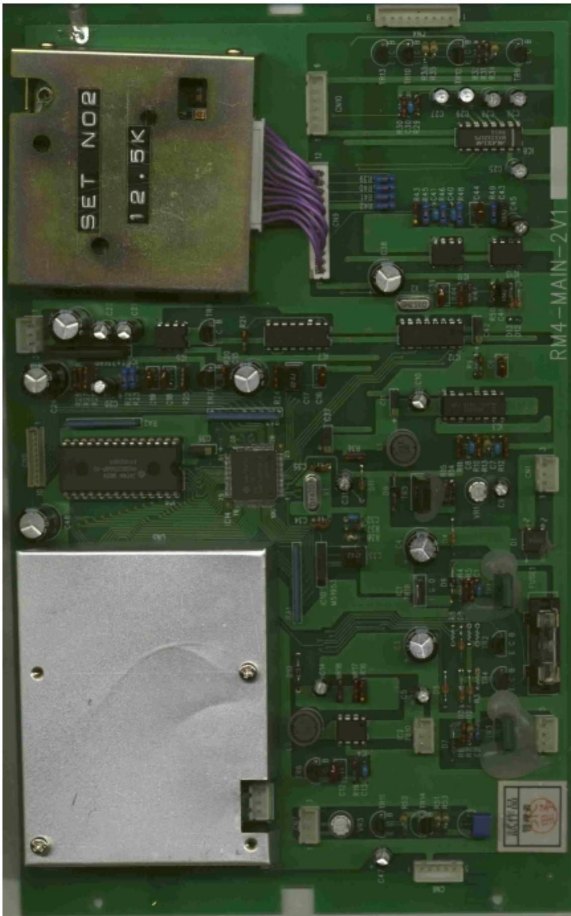
Processor Board.
