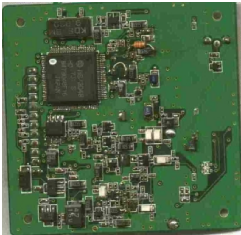
Receiver Board: Foil side
