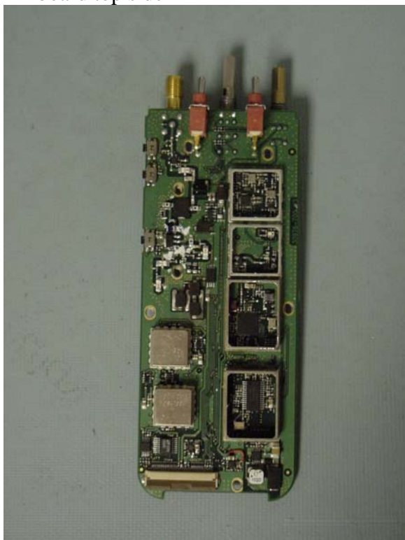
RF board top side
