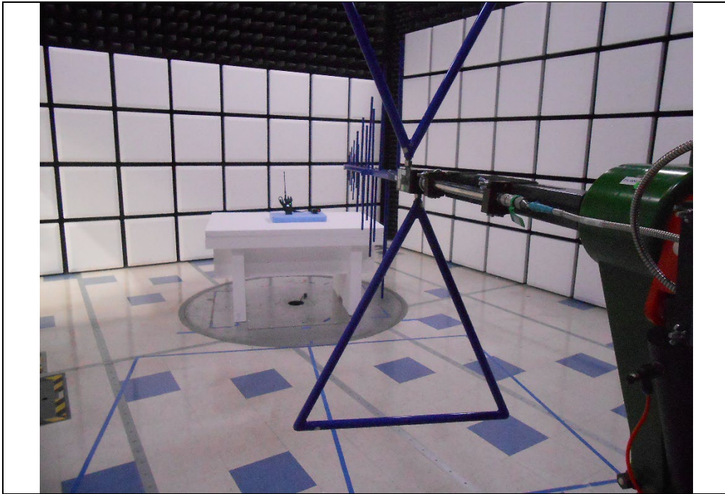
RF Radiated_ Below 1 GHz
