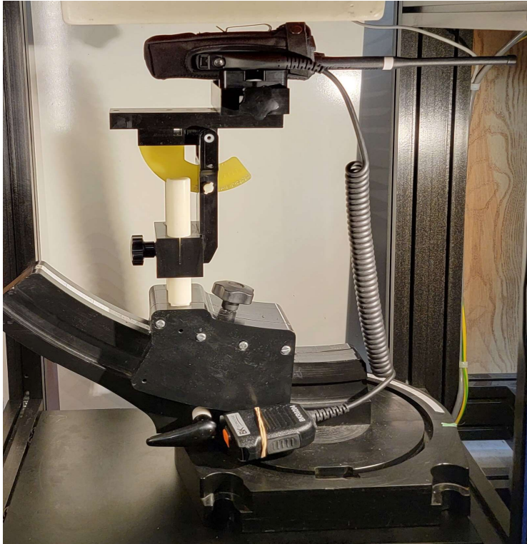
Figure C.4 Test Setup - Body, Plot B60, B61, B82 – D1, P1, T1, A1 – Close View
