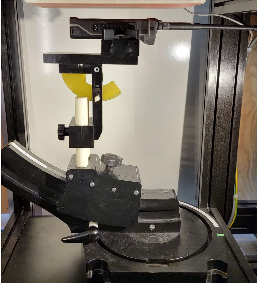
Figure C.6 Test Setup - Face, Plot F55, F56, F81 – Close View
