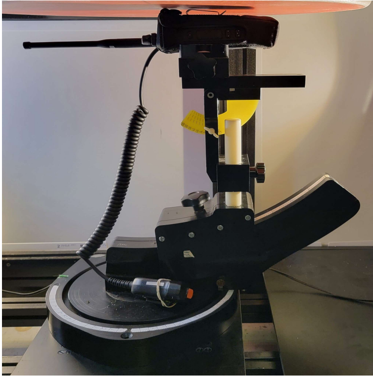
Figure C.2 Test Setup - Body, Plot B2 – D1, P1, T2, A1 – Close View
