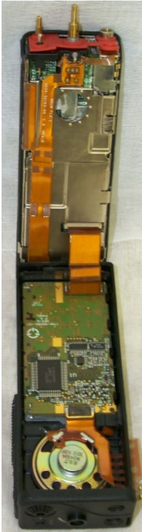
Photo 6. EUT, Case Opened
