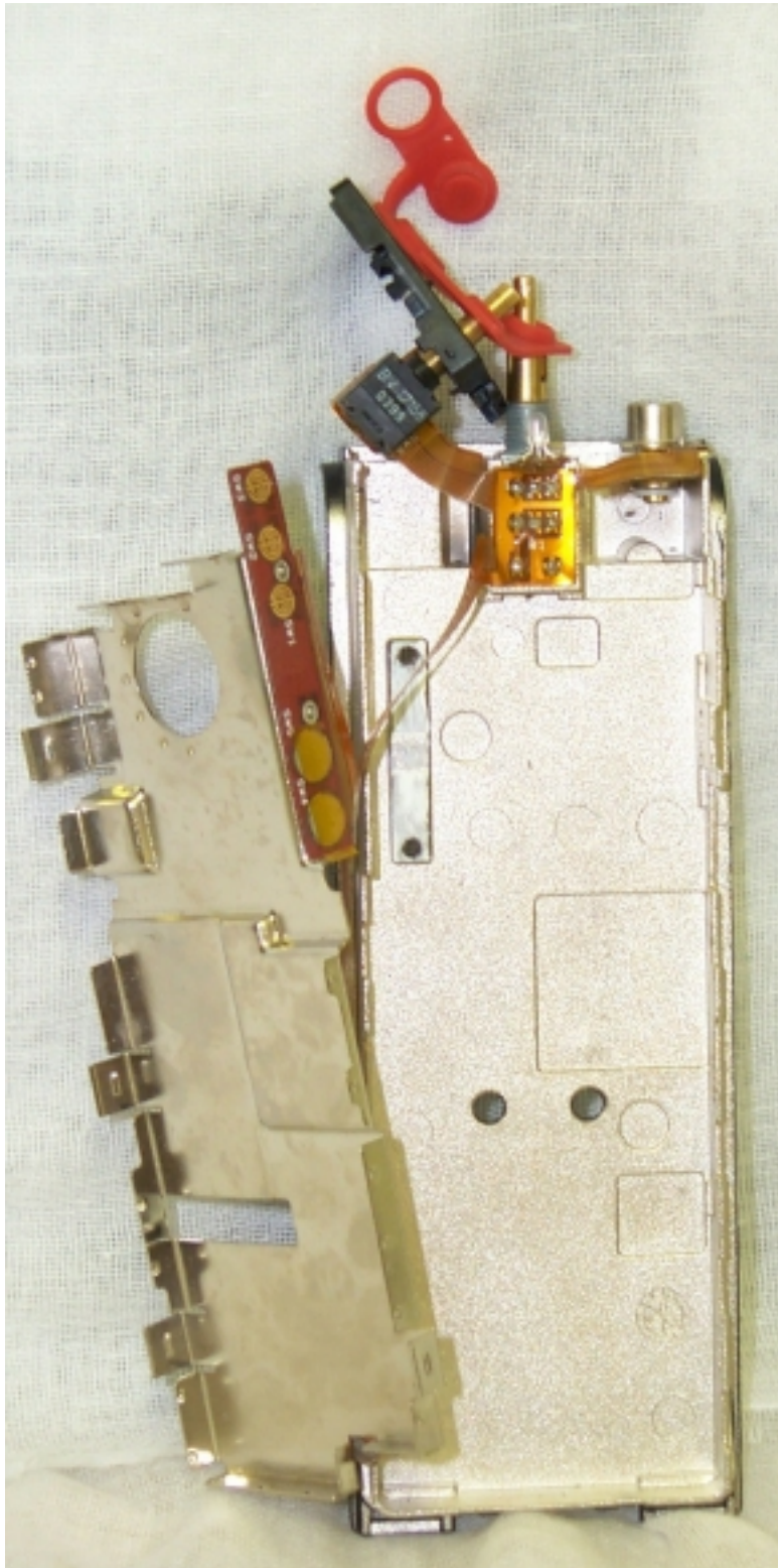
Photo 12. EUT, View Showing Main PCB Removed
