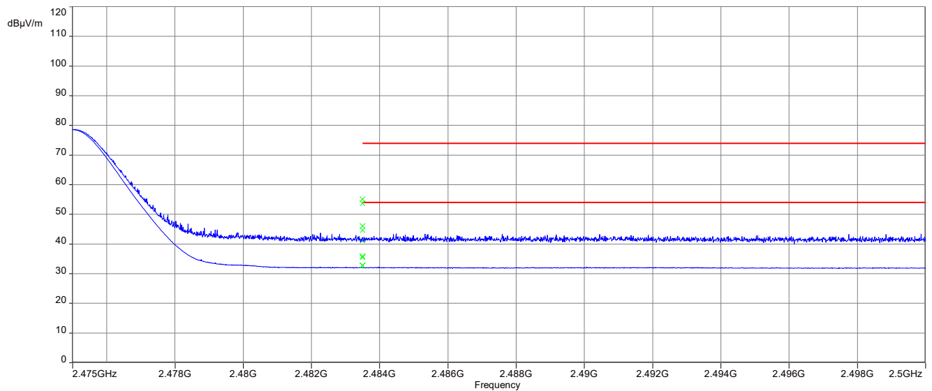
Plot 2: Upper restricted band, 2G4 DIPOLE ANTENNA (~200 mm), Prot-002
