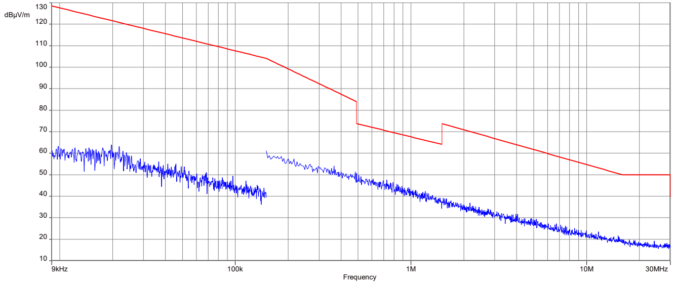
Plot 3: 9 kHz to 30 MHz, 2475 MHz, transmit mode, 2G4 DIPOLE ANTENNA (~200 mm), Prot-002
