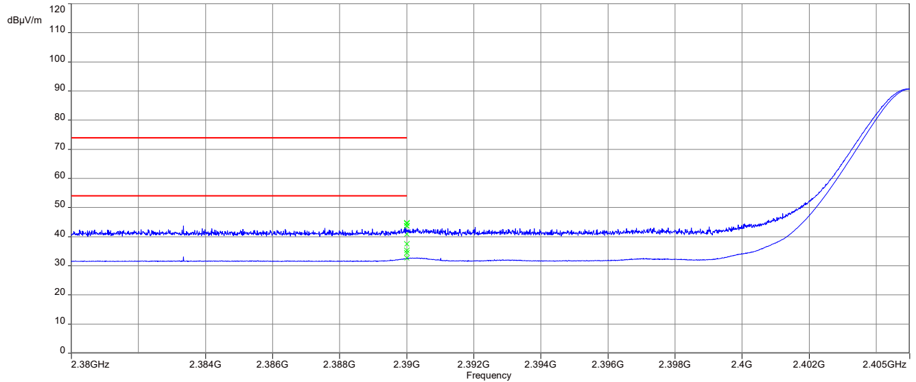
Plot 3: Lower restricted band, 2G4 DIPOLE ANTENNA (~120 mm), Prot-001
