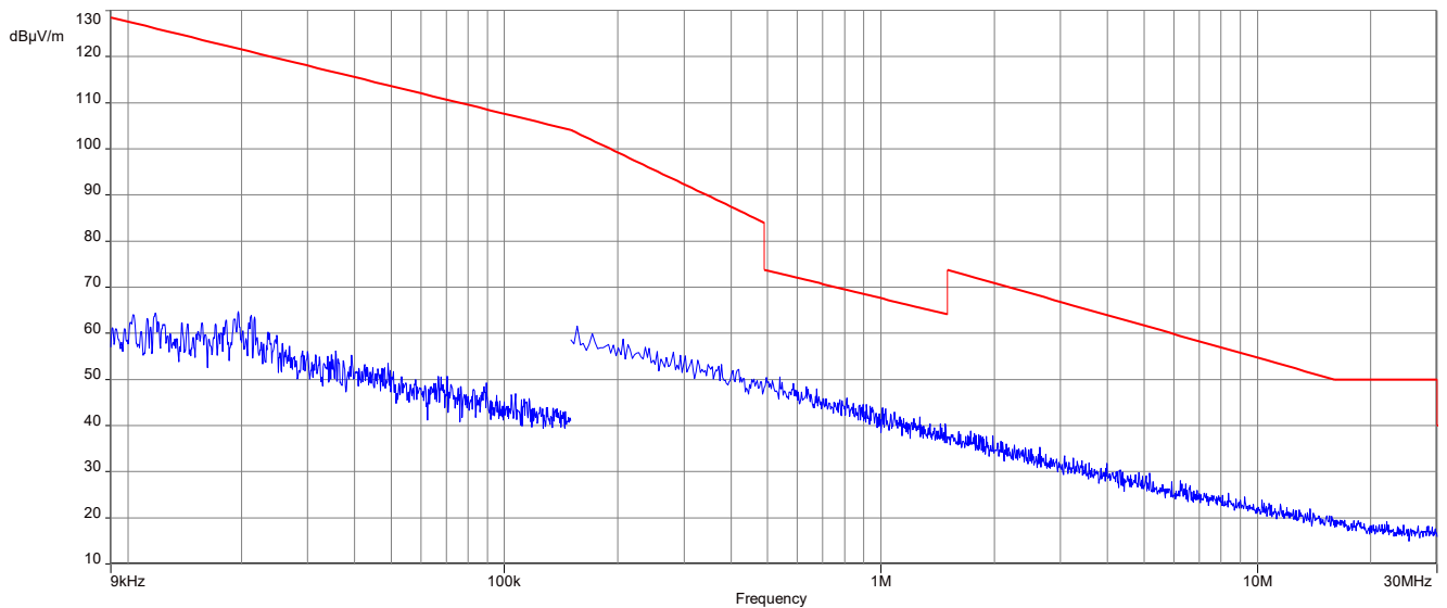
Plot 4: 9 kHz to 30 MHz, 2405 MHz, transmit mode, 2G4 DIPOLE ANTENNA (~120 mm), Prot-001
