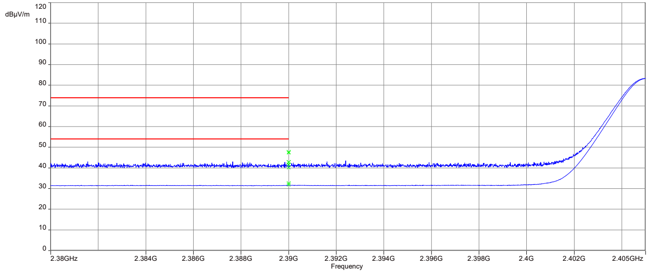
Plot 5: Lower restricted band, BOA24008NF ANTENNA, OMNI, Prot-001
