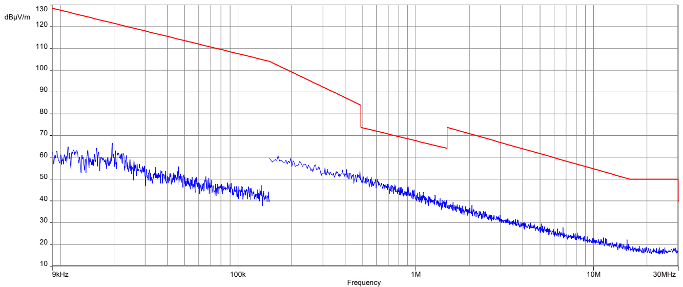
Plot 8: 9 kHz to 30 MHz, 2440 MHz, transmit mode, BOA24008NF ANTENNA, OMNI, Prot-001
