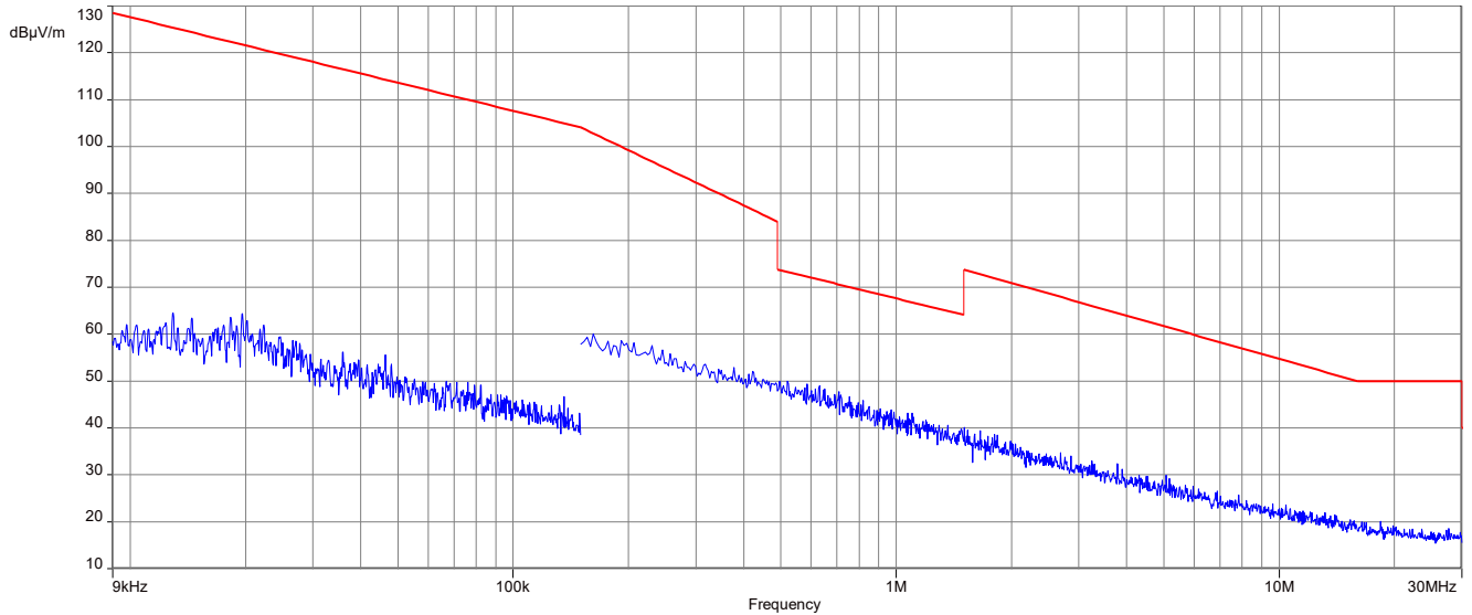
Plot 5: 9 kHz to 30 MHz, 2440 MHz, transmit mode, 2G4 DIPOLE ANTENNA (~120 mm), Prot-001
