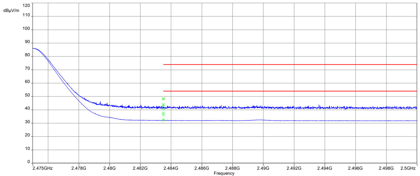
Plot 6: Upper restricted band, BOA24008NF ANTENNA, OMNI, Prot-001
