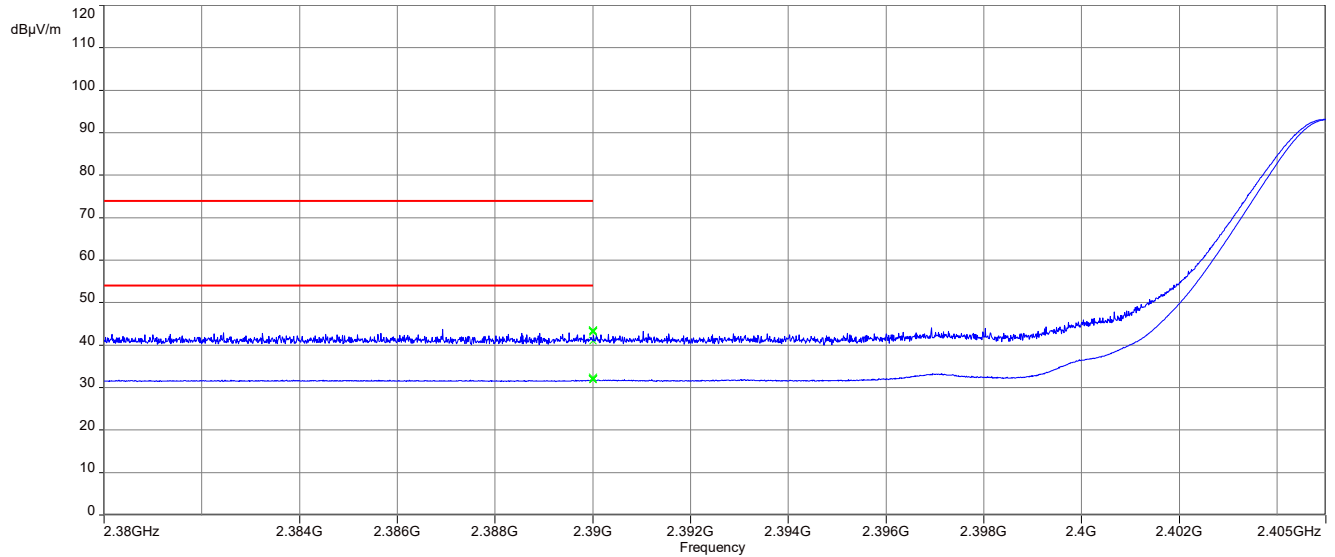
Plot 1: Lower restricted band, 2G4 DIPOLE ANTENNA (~200 mm), Prot-002
