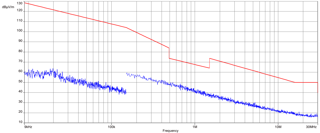
Plot 1: 9 kHz to 30 MHz, 2405 MHz, transmit mode, 2G4 DIPOLE ANTENNA (~200 mm), Prot-002
