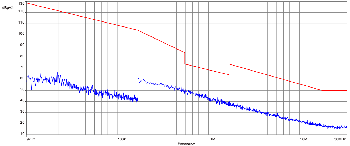
Plot 9: 9 kHz to 30 MHz, 2475 MHz, transmit mode, BOA24008NF ANTENNA, OMNI, Prot-001
