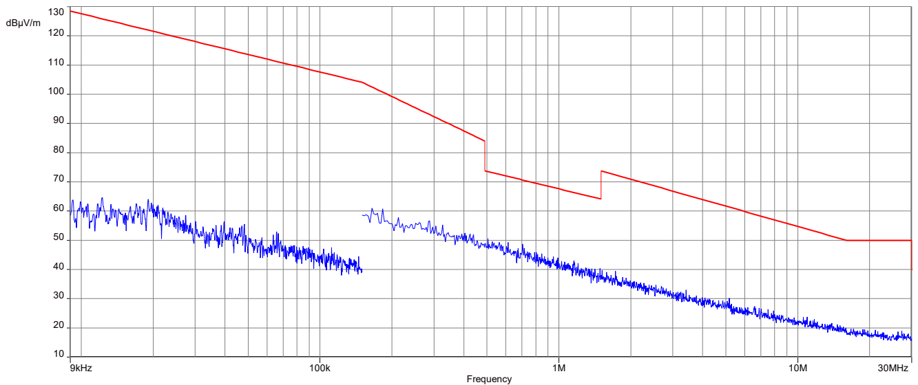
Plot 2: 9 kHz to 30 MHz, 2440 MHz, transmit mode, 2G4 DIPOLE ANTENNA (~200 mm), Prot-002
