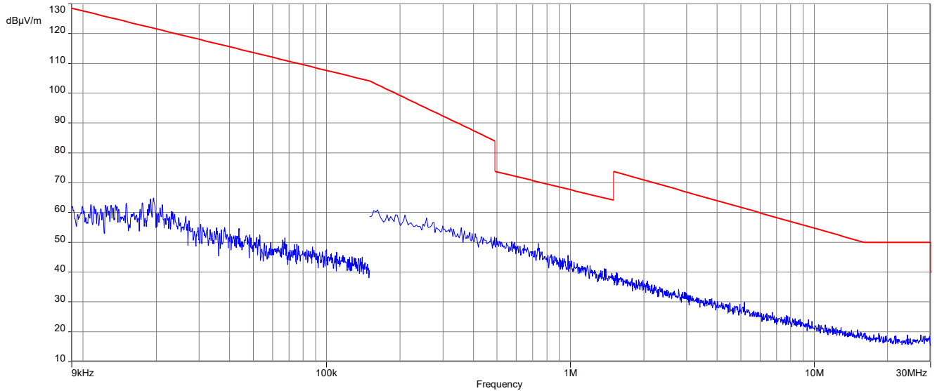
Plot 7: 9 kHz to 30 MHz, 2405 MHz, transmit mode, BOA24008NF ANTENNA, OMNI, Prot-001
