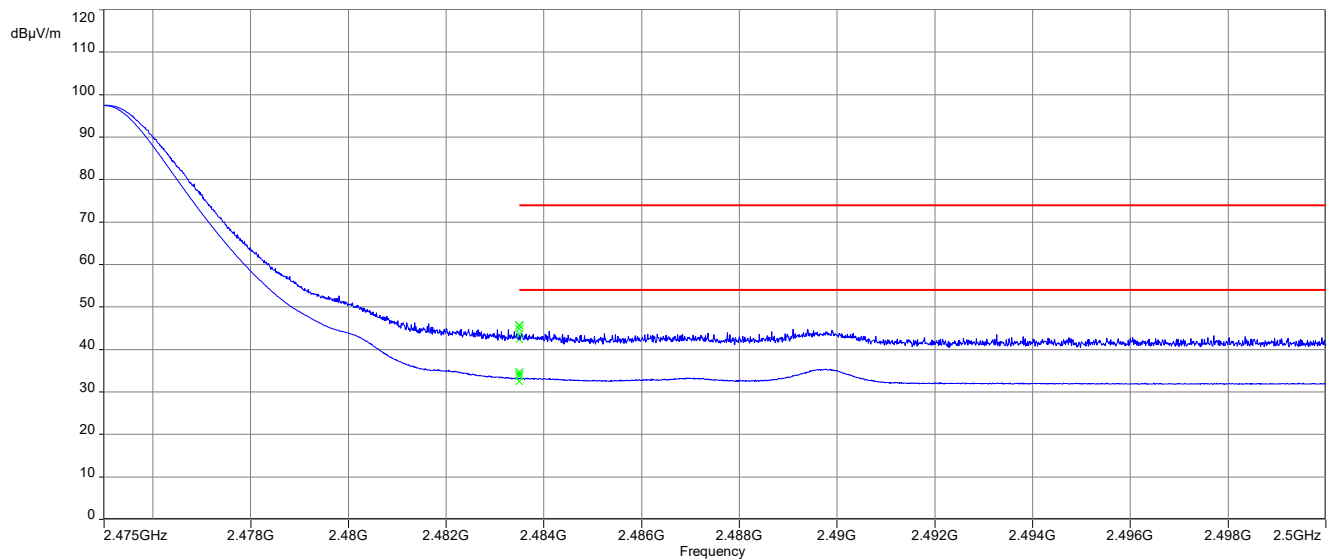
Plot 4: Upper restricted band, 2G4 DIPOLE ANTENNA (~120 mm), Prot-001
