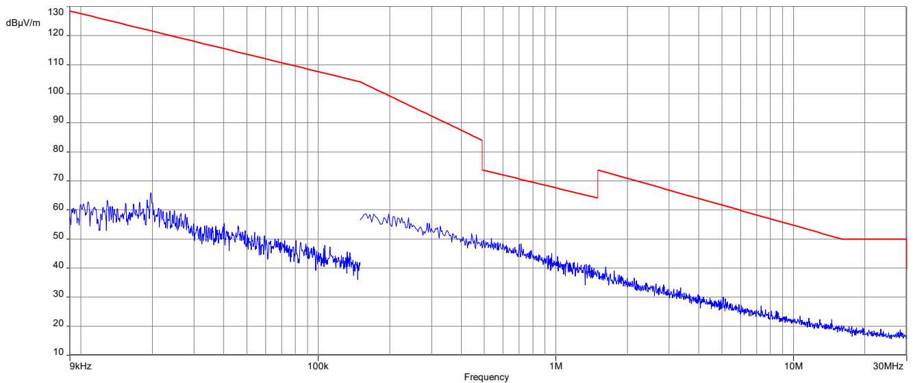
Plot 6: 9 kHz to 30 MHz, 2475 MHz, transmit mode, 2G4 DIPOLE ANTENNA (~120 mm), Prot-001
