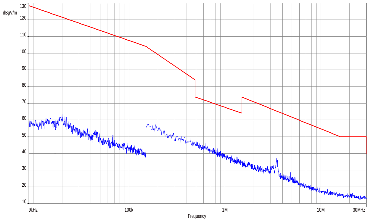
Plot 1: 9 kHz – 30 MHz, special test mode, f_{\text{low}}/f_{\text{mid}}/f_{\text{high}}
