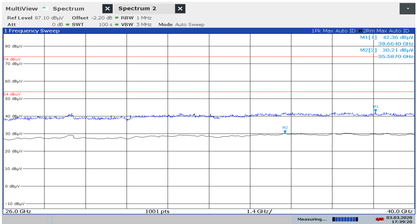
Plot 5: 26 GHz – 40 GHz, PEAK/RMS-measurement, f_{\text{low}}/f_{\text{mid}}/f_{\text{high}}
