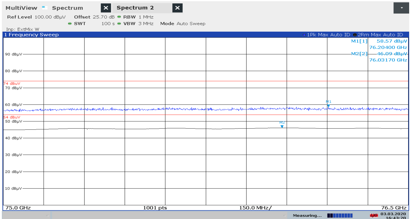
Plot 8: 75 GHz – 76.5 GHz, PEAK/RMS-measurement, f_{\text{low}}/f_{\text{mid}}/f_{\text{high}}
