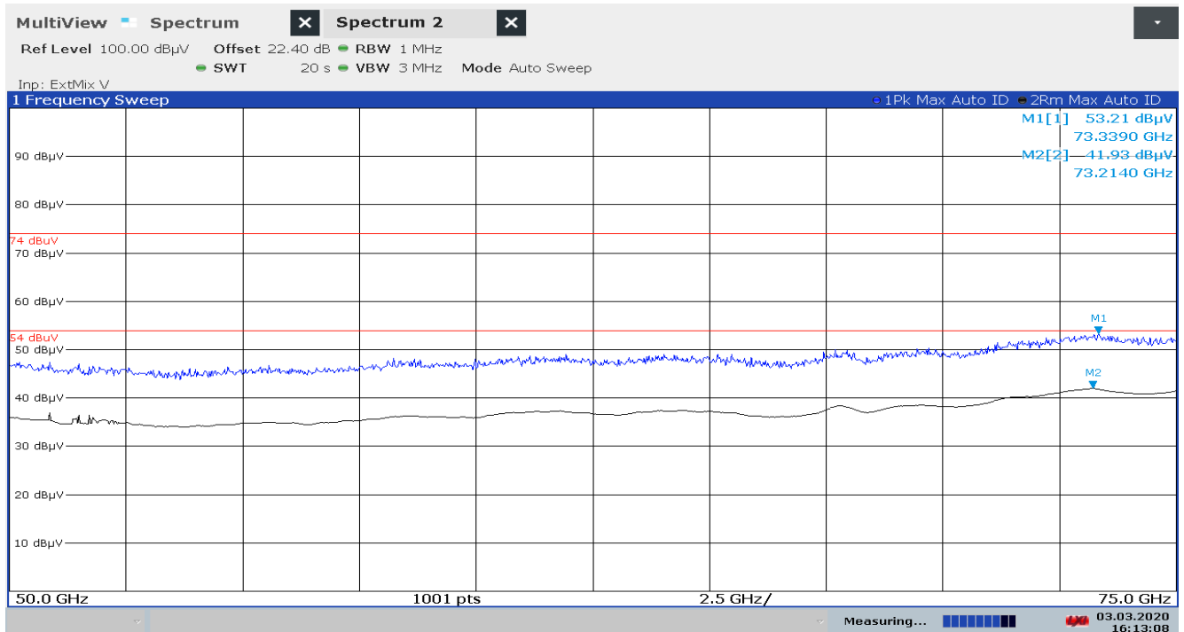
Plot 7: 50 GHz – 75 GHz, PEAK/RMS-measurement, f_{\text{low}}/f_{\text{mid}}/f_{\text{high}}
