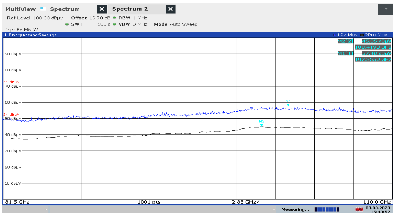
Plot 10: 81.5 GHz – 110 GHz, PEAK/RMS-measurement, f_{\text{low}}/f_{\text{mid}}/f_{\text{high}}
