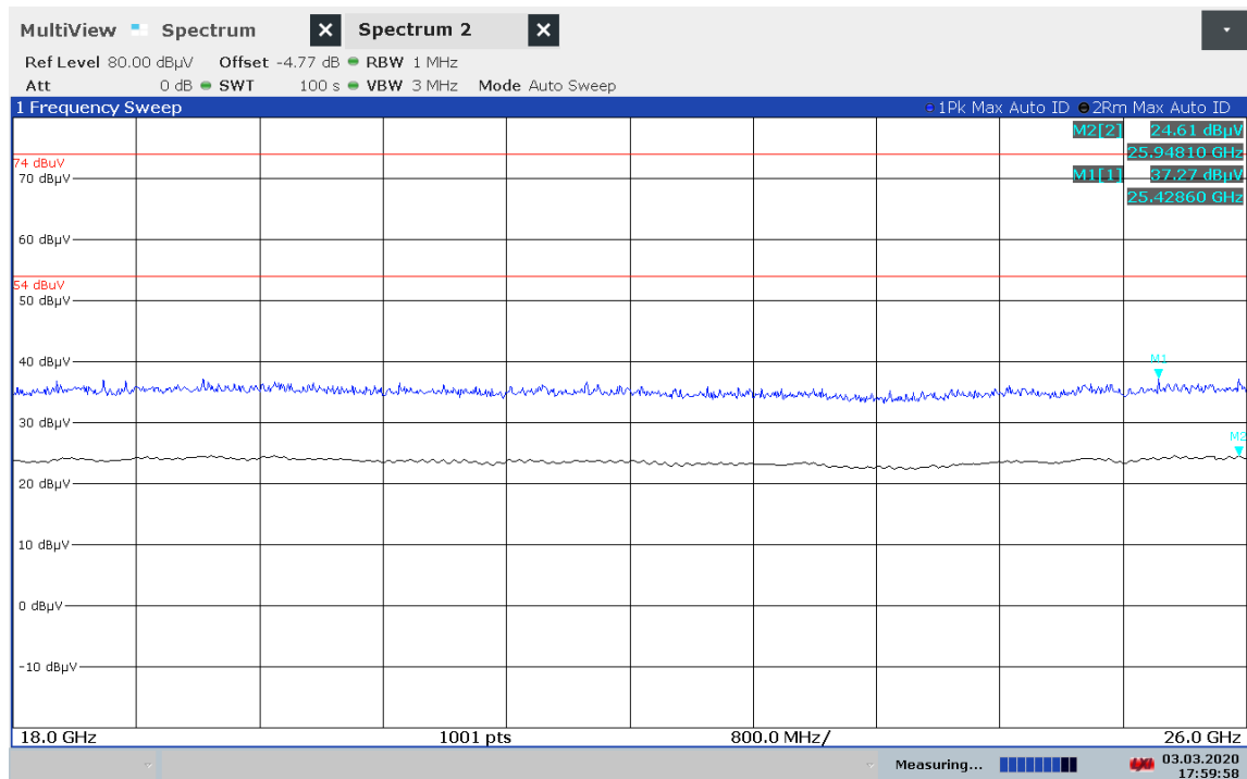
Plot 4: 18 GHz – 26 GHz, PEAK/RMS-measurement, f_{\text{low}}/f_{\text{mid}}/f_{\text{high}}
