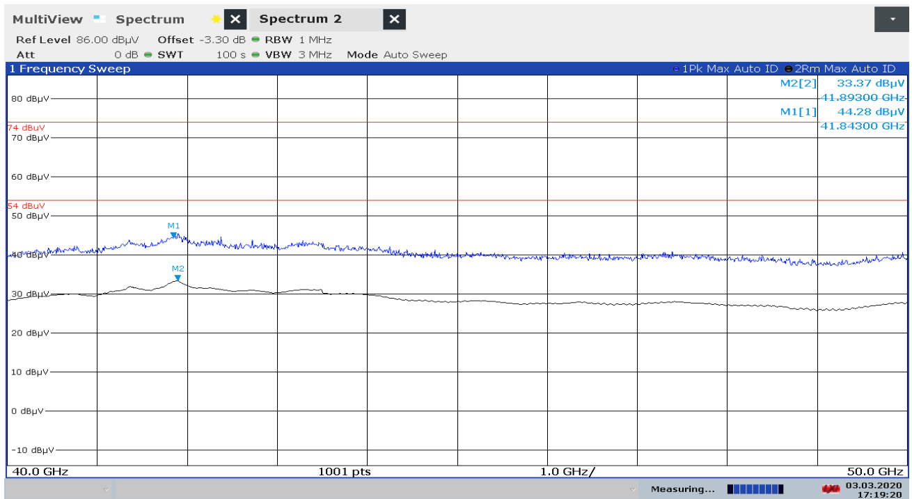
Plot 6: 40 GHz – 50 GHz, PEAK/RMS-measurement, f_{\text{low}}/f_{\text{mid}}/f_{\text{high}}
