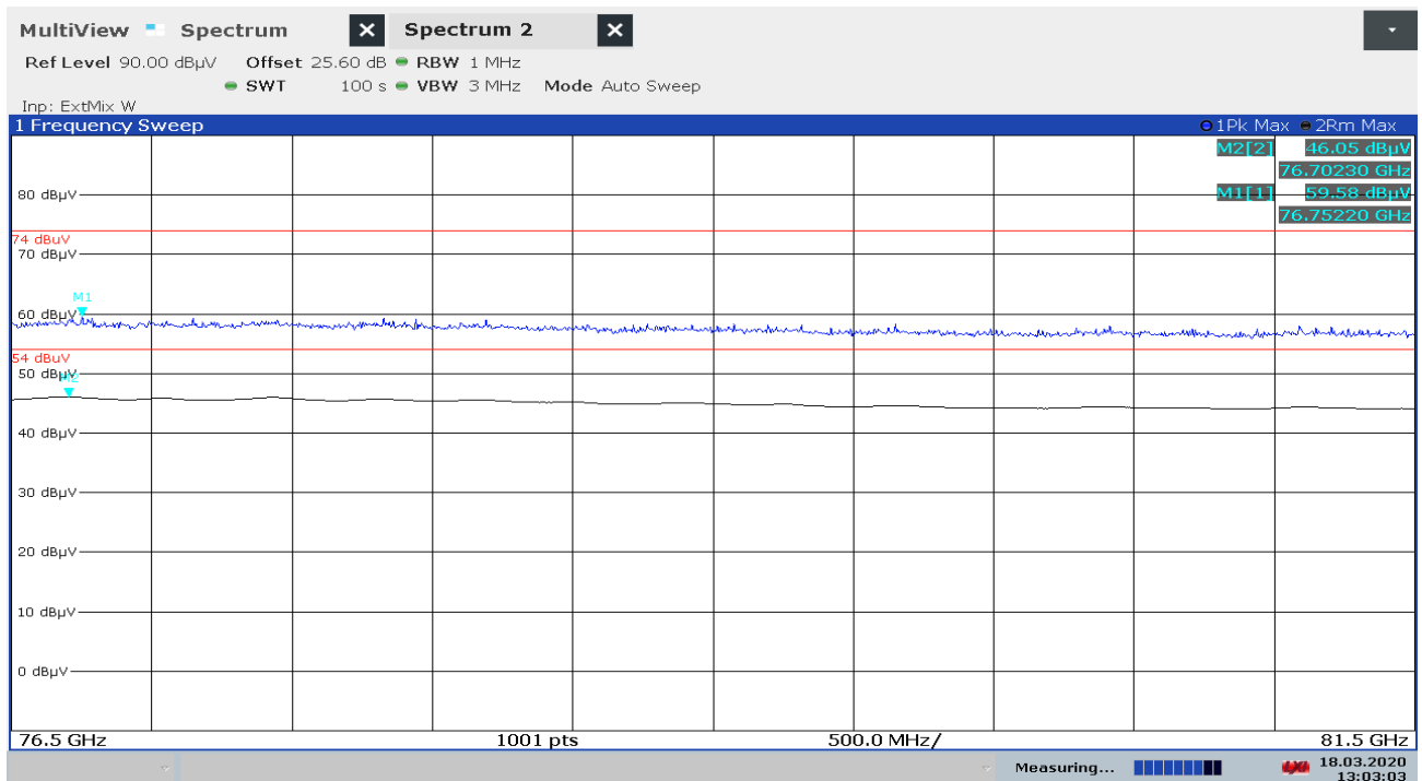
Plot 9: 76.5 GHz – 81.5 GHz, PEAK/RMS-measurement, f_{\text{low}}/f_{\text{mid}}/f_{\text{high}}
