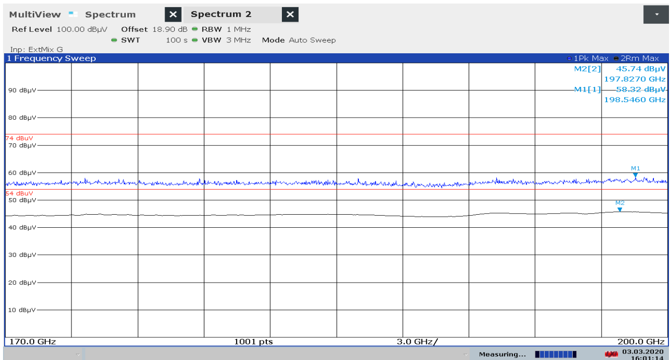
Plot 12: 170 GHz – 200 GHz, PEAK/RMS-measurement, f_{\text{low}}/f_{\text{mid}}/f_{\text{high}}
