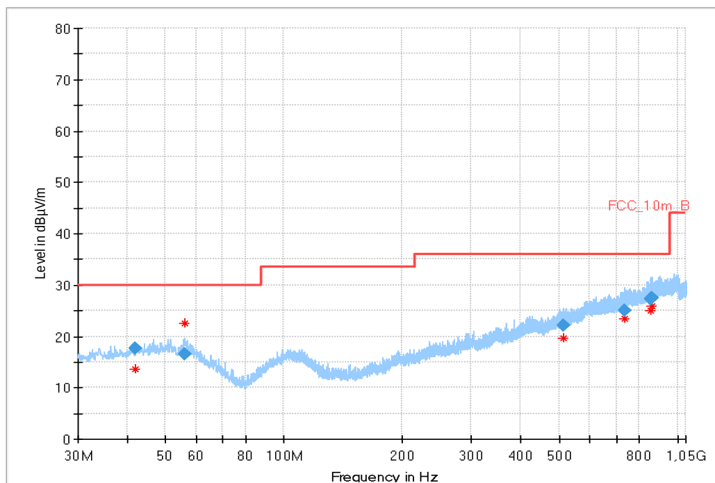
Plot 2: 30 MHz – 1000 MHz, special test mode, f_{\text{low}}/f_{\text{mid}}/f_{\text{high}}
