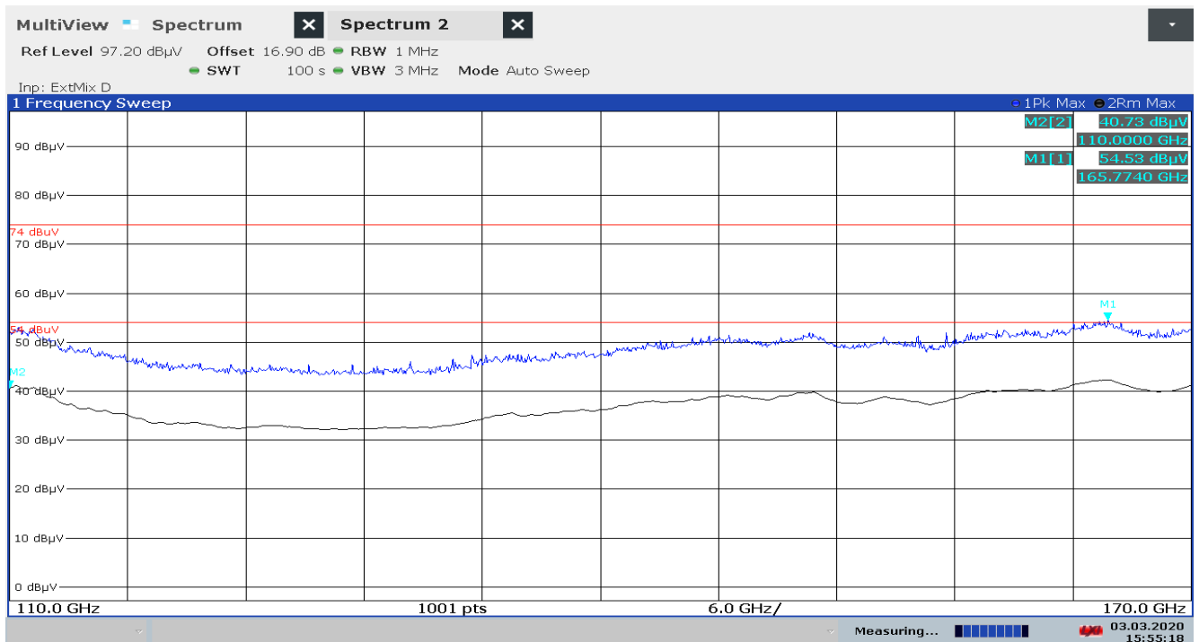
Plot 11: 110 GHz – 170 GHz, PEAK/RMS-measurement, f_{\text{low}}/f_{\text{mid}}/f_{\text{high}}
